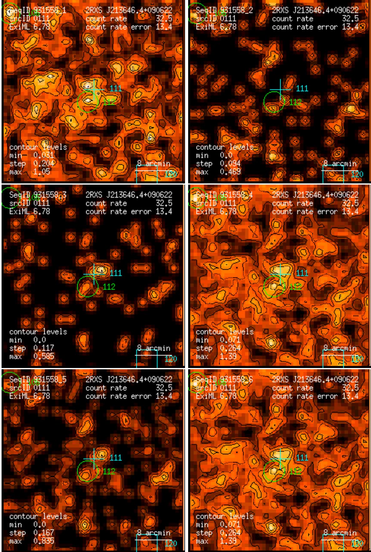
Figure 111: RASS 931558: detection 0111: band rate images, Gaussian filter: (1) PSPC channels 11 – 41, (2) 52 – 90, (3) 91 – 201, (4) 11 – 235, (5) 52 – 201, (6) 11 – 201. Broad band rates in counts/ks. Band rate contour levels in counts/ks/arcmin 2 .
