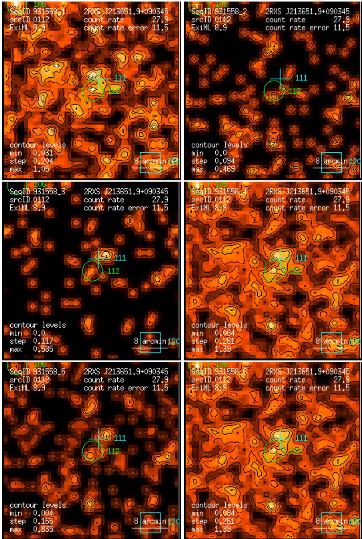
Figure 112: RASS 931558: detection 0112: band rate images, Gaussian filter: (1) PSPC channels 11 – 41, (2) 52 – 90, (3) 91 – 201, (4) 11 – 235, (5) 52 – 201, (6) 11 – 201. Broad band rates in counts/ks. Band rate contour levels in counts/ks/arcmin 2 .
