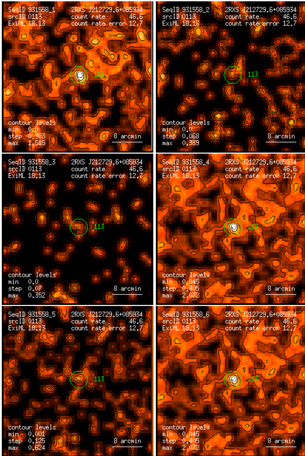
Figure 113: RASS 931558: detection 0113: band rate images, Gaussian filter: (1) PSPC channels 11 – 41, (2) 52 – 90, (3) 91 – 201, (4) 11 – 235, (5) 52 – 201, (6) 11 – 201. Broad band rates in counts/ks. Band rate contour levels in counts/ks/arcmin 2 .
