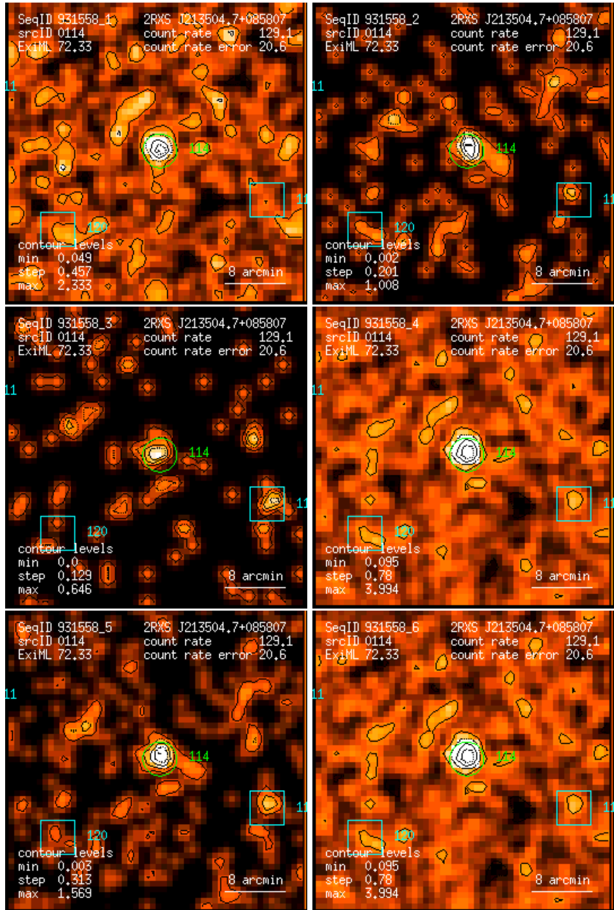
Figure 114: RASS 931558: detection 0114: band rate images, Gaussian filter: (1) PSPC channels 11 – 41, (2) 52 – 90, (3) 91 – 201, (4) 11 – 235, (5) 52 – 201, (6) 11 – 201. Broad band rates in counts/ks. Band rate contour levels in counts/ks/arcmin 2 .
