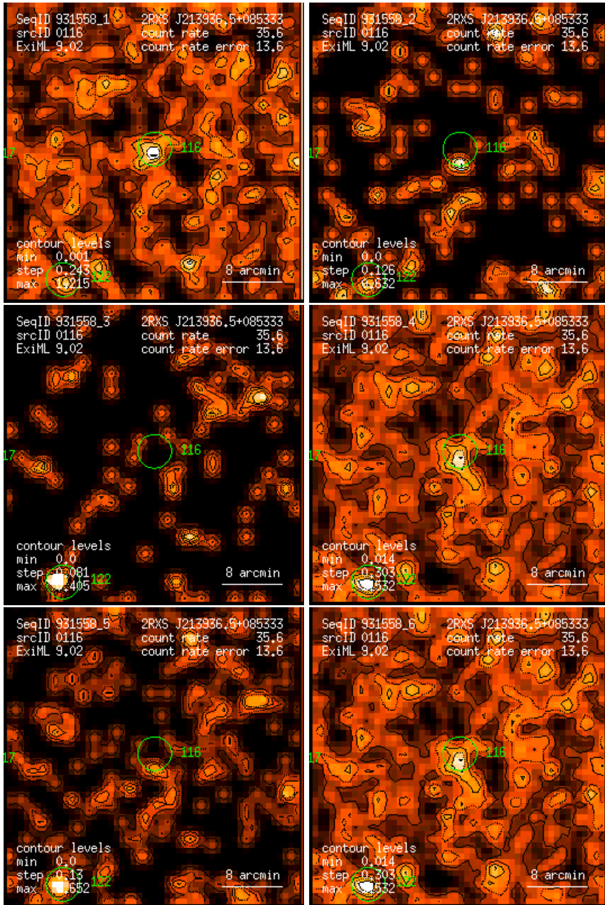
Figure 116: RASS 931558: detection 0116: band rate images, Gaussian filter: (1) PSPC channels 11 – 41, (2) 52 – 90, (3) 91 – 201, (4) 11 – 235, (5) 52 – 201, (6) 11 – 201. Broad band rates in counts/ks. Band rate contour levels in counts/ks/arcmin 2 .
