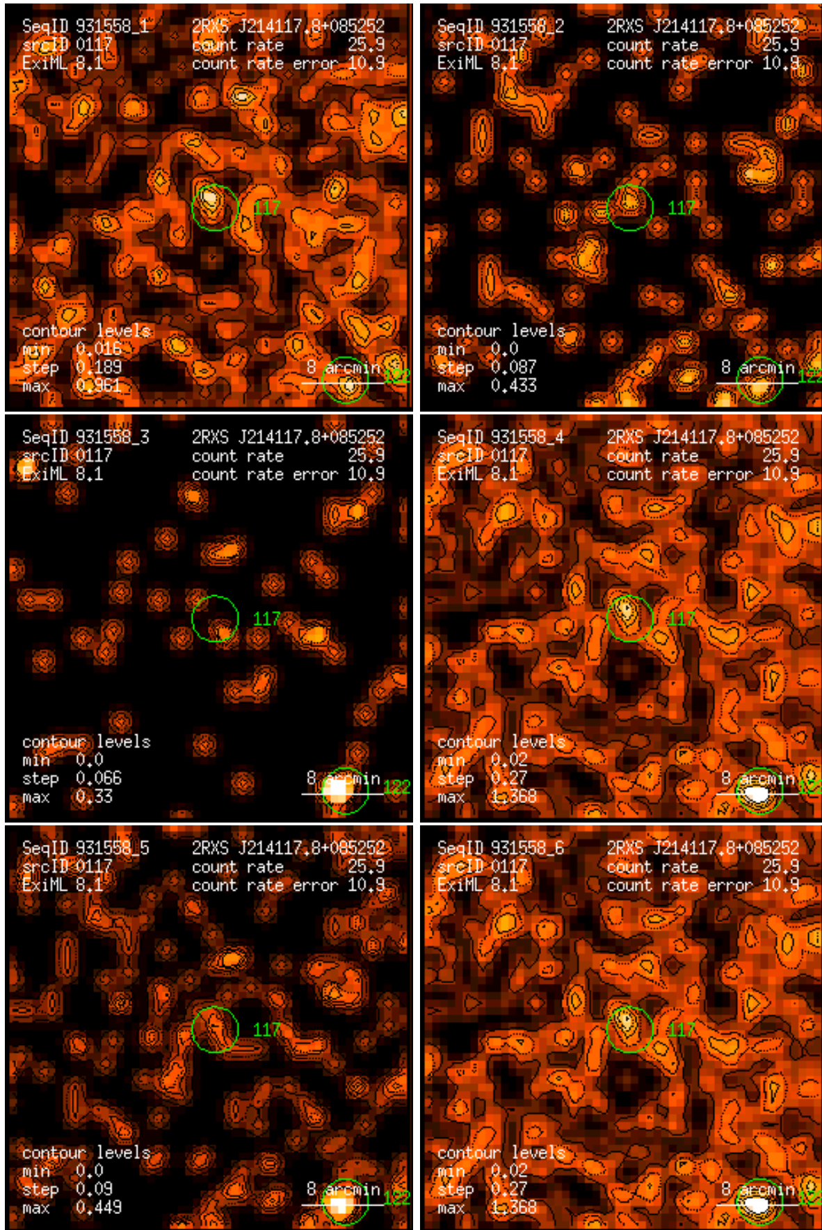
Figure 117: RASS 931558: detection 0117: band rate images, Gaussian filter: (1) PSPC channels 11 – 41, (2) 52 – 90, (3) 91 – 201, (4) 11 – 235, (5) 52 – 201, (6) 11 – 201. Broad band rates in counts/ks. Band rate contour levels in counts/ks/arcmin 2 .
