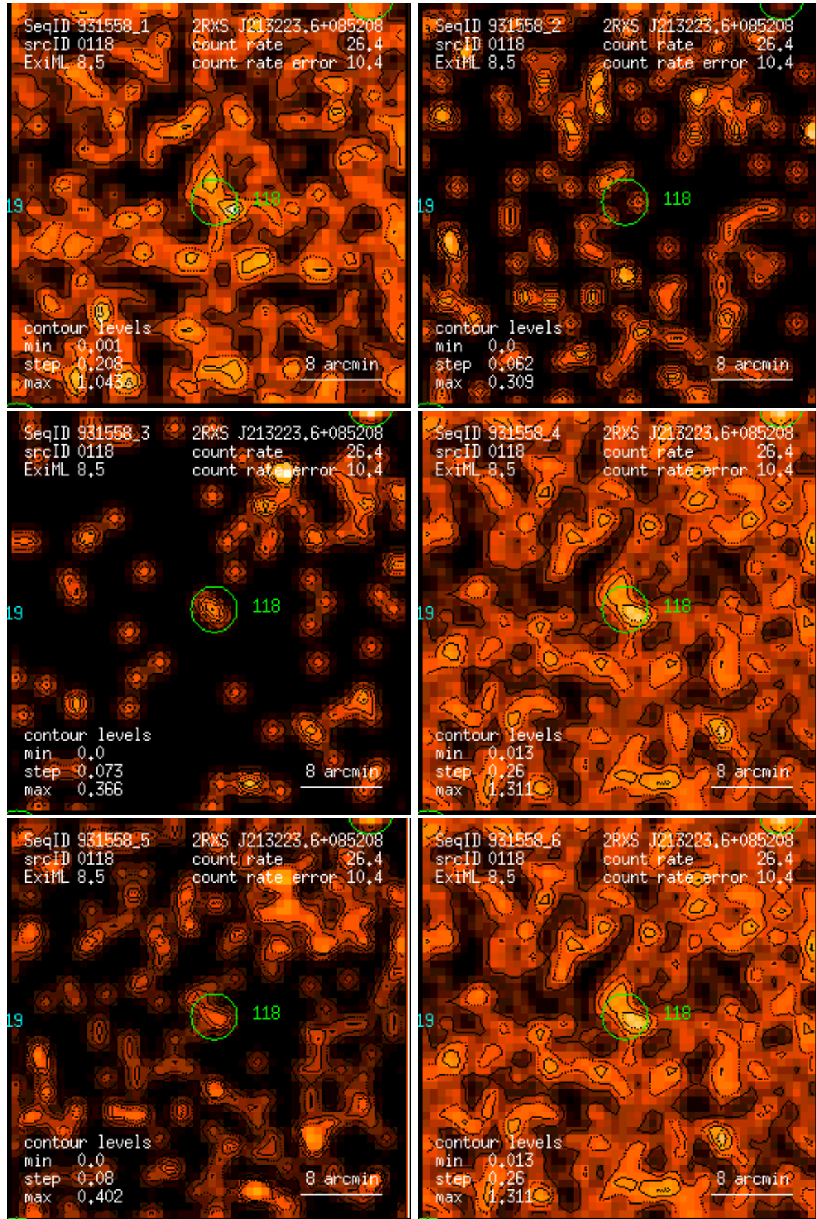
Figure 118: RASS 931558: detection 0118: band rate images, Gaussian filter: (1) PSPC channels 11 – 41, (2) 52 – 90, (3) 91 – 201, (4) 11 – 235, (5) 52 – 201, (6) 11 – 201. Broad band rates in counts/ks. Band rate contour levels in counts/ks/arcmin 2 .
