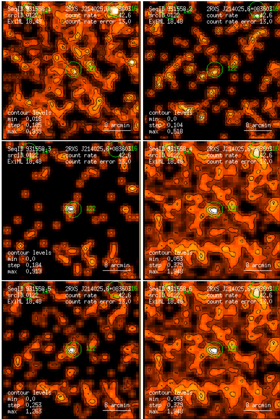
Figure 122: RASS 931558: detection 0122: band rate images, Gaussian filter: (1) PSPC channels 11 – 41, (2) 52 – 90, (3) 91 – 201, (4) 11 – 235, (5) 52 – 201, (6) 11 – 201. Broad band rates in counts/ks. Band rate contour levels in counts/ks/arcmin 2 .
