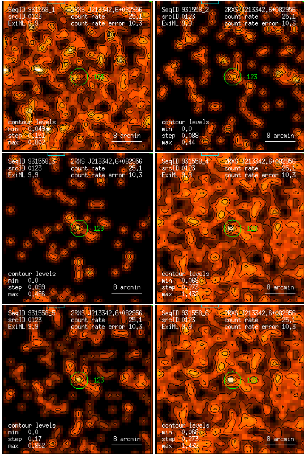
Figure 123: RASS 931558: detection 0123: band rate images, Gaussian filter: (1) PSPC channels 11 – 41, (2) 52 – 90, (3) 91 – 201, (4) 11 – 235, (5) 52 – 201, (6) 11 – 201. Broad band rates in counts/ks. Band rate contour levels in counts/ks/arcmin 2 .
