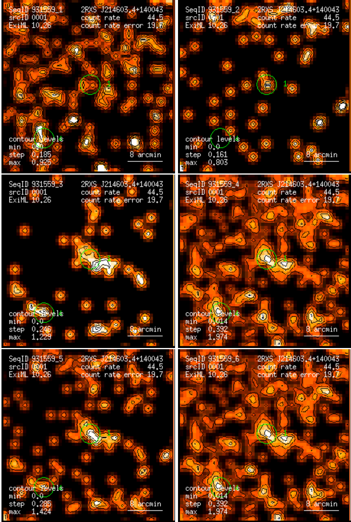
Figure 1: RASS 931559: detection 0001: band rate images, Gaussian filter: (1) PSPC channels 11 – 41, (2) 52 – 90, (3) 91 – 201, (4) 11 – 235, (5) 52 – 201, (6) 11 – 201. Broad band rates in counts/ks. Band rate contour levels in counts/ks/arcmin 2 .
