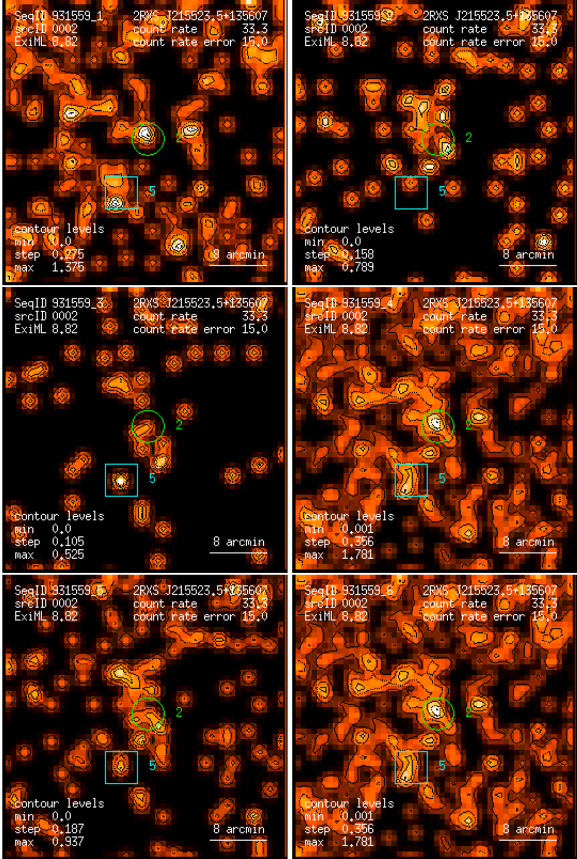
Figure 2: RASS 931559: detection 0002: band rate images, Gaussian filter: (1) PSPC channels 11 – 41, (2) 52 – 90, (3) 91 – 201, (4) 11 – 235, (5) 52 – 201, (6) 11 – 201. Broad band rates in counts/ks. Band rate contour levels in counts/ks/arcmin 2 .
