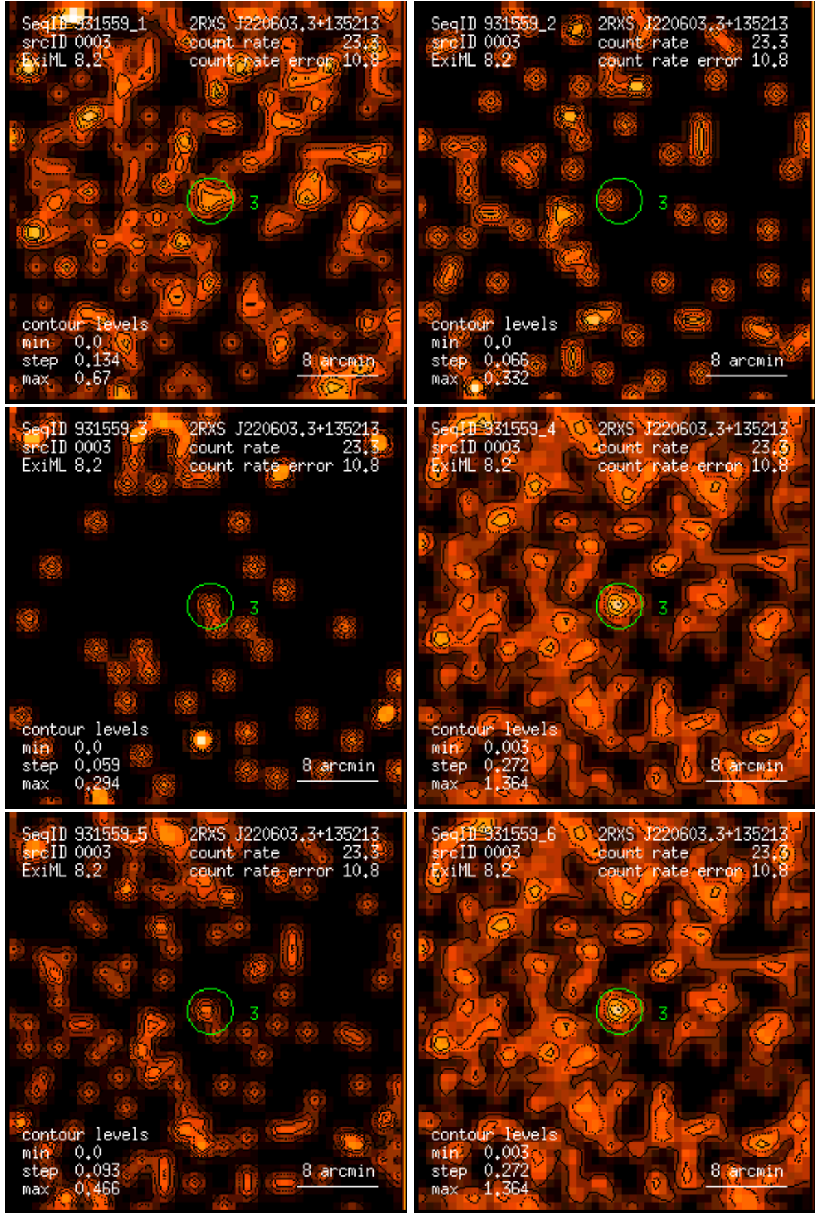
Figure 3: RASS 931559: detection 0003: band rate images, Gaussian filter: (1) PSPC channels 11 – 41, (2) 52 – 90, (3) 91 – 201, (4) 11 – 235, (5) 52 – 201, (6) 11 – 201. Broad band rates in counts/ks. Band rate contour levels in counts/ks/arcmin 2 .
