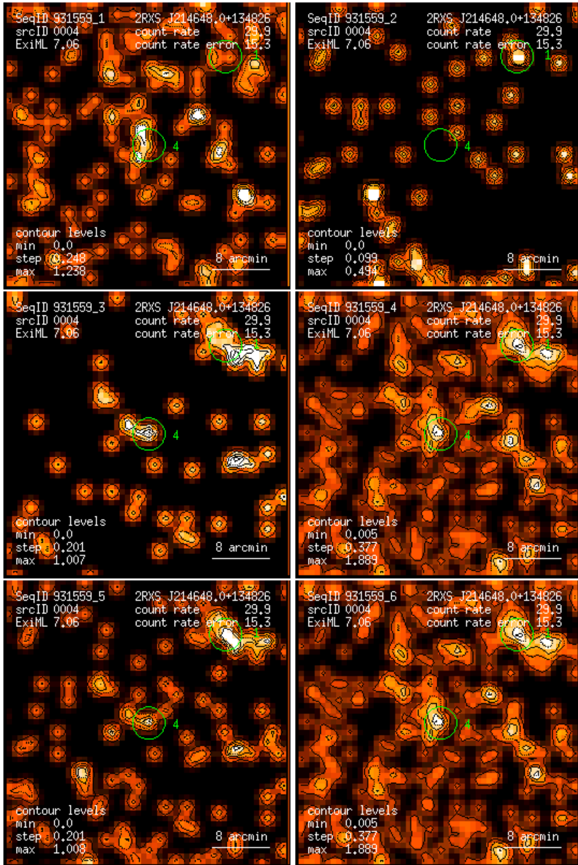
Figure 4: RASS 931559: detection 0004: band rate images, Gaussian filter: (1) PSPC channels 11 – 41, (2) 52 – 90, (3) 91 – 201, (4) 11 – 235, (5) 52 – 201, (6) 11 – 201. Broad band rates in counts/ks. Band rate contour levels in counts/ks/arcmin 2 .
