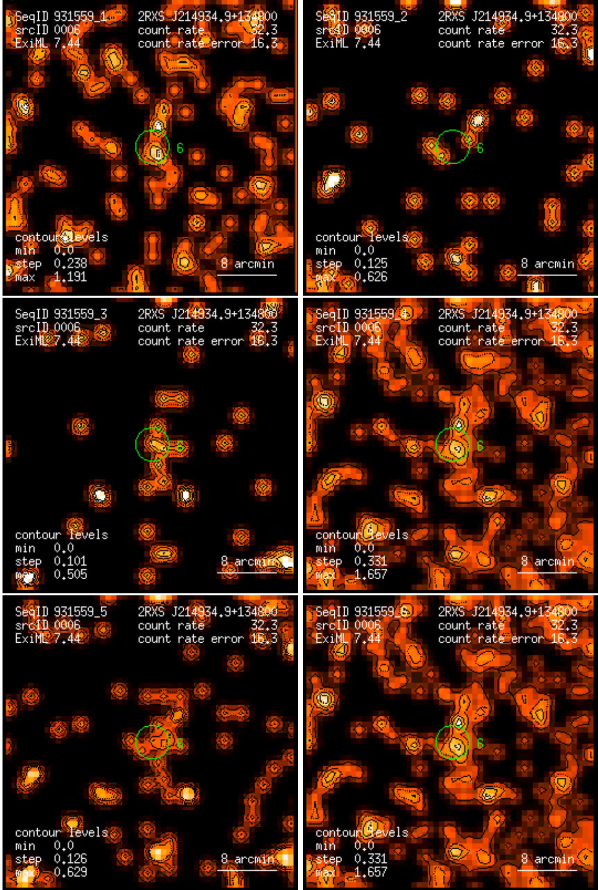
Figure 6: RASS 931559: detection 0006: band rate images, Gaussian filter: (1) PSPC channels 11 – 41, (2) 52 – 90, (3) 91 – 201, (4) 11 – 235, (5) 52 – 201, (6) 11 – 201. Broad band rates in counts/ks. Band rate contour levels in counts/ks/arcmin 2 .
