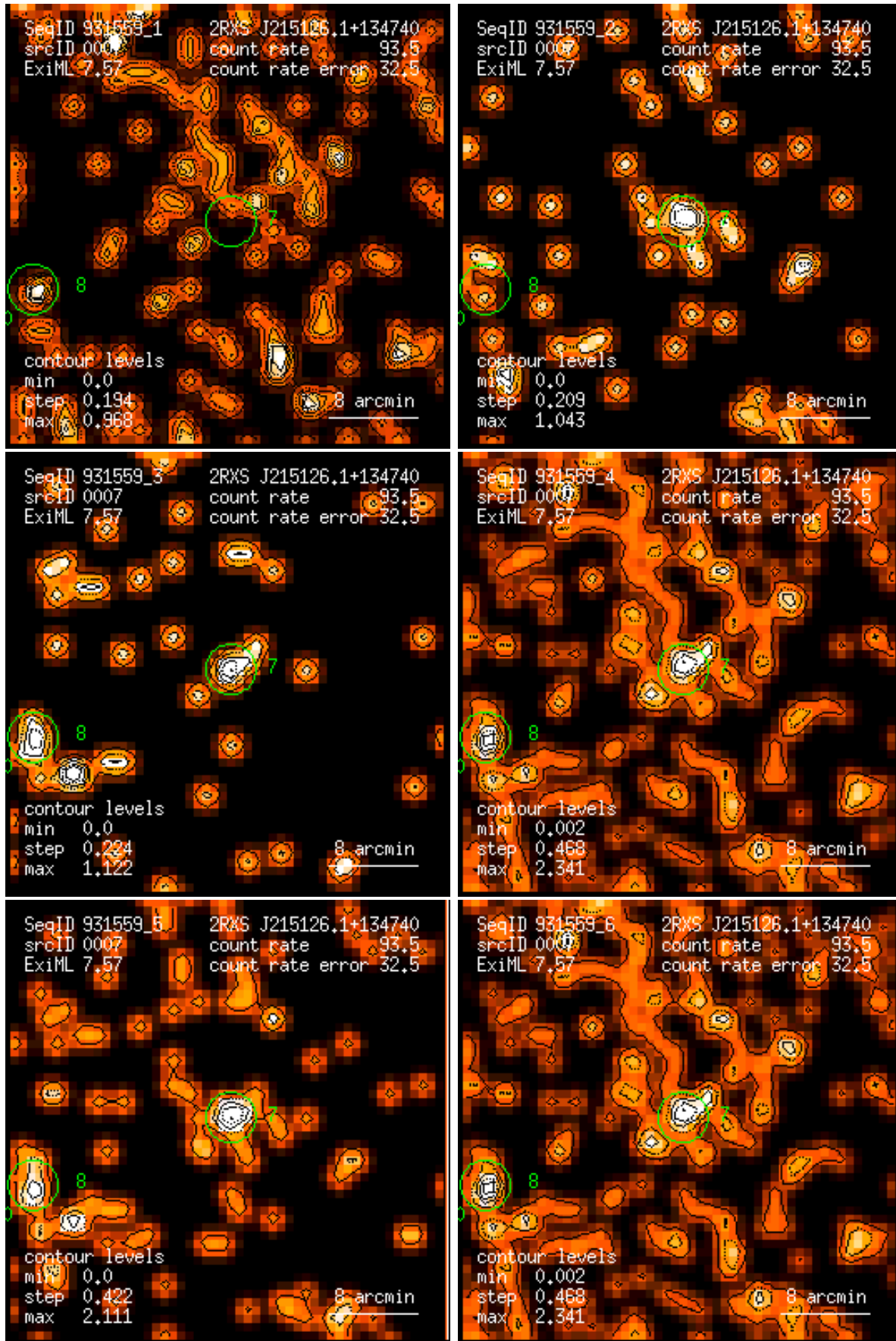
Figure 7: RASS 931559: detection 0007: band rate images, Gaussian filter: (1) PSPC channels 11 – 41, (2) 52 – 90, (3) 91 – 201, (4) 11 – 235, (5) 52 – 201, (6) 11 – 201. Broad band rates in counts/ks. Band rate contour levels in counts/ks/arcmin 2 .
