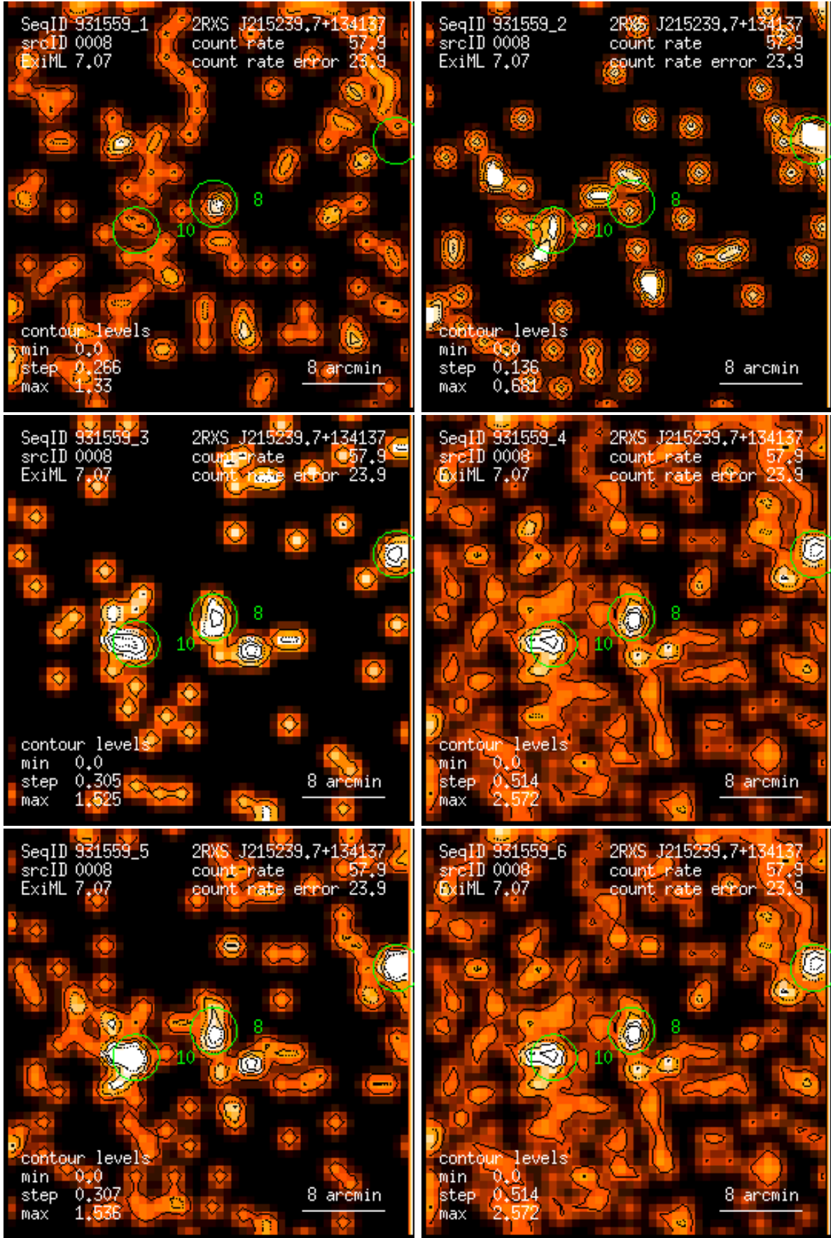
Figure 8: RASS 931559: detection 0008: band rate images, Gaussian filter: (1) PSPC channels 11 – 41, (2) 52 – 90, (3) 91 – 201, (4) 11 – 235, (5) 52 – 201, (6) 11 – 201. Broad band rates in counts/ks. Band rate contour levels in counts/ks/arcmin 2 .
