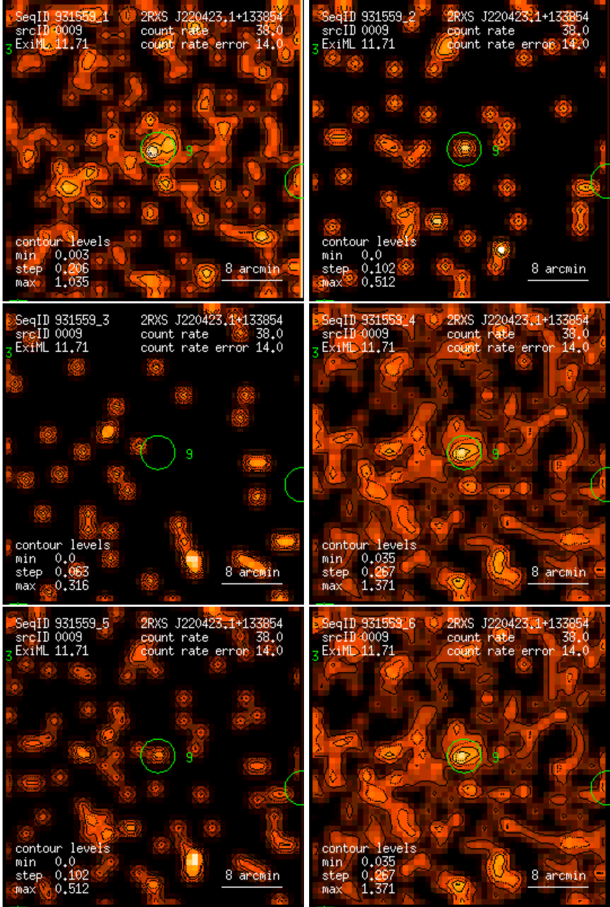
Figure 9: RASS 931559: detection 0009: band rate images, Gaussian filter: (1) PSPC channels 11 – 41, (2) 52 – 90, (3) 91 – 201, (4) 11 – 235, (5) 52 – 201, (6) 11 – 201. Broad band rates in counts/ks. Band rate contour levels in counts/ks/arcmin 2 .
