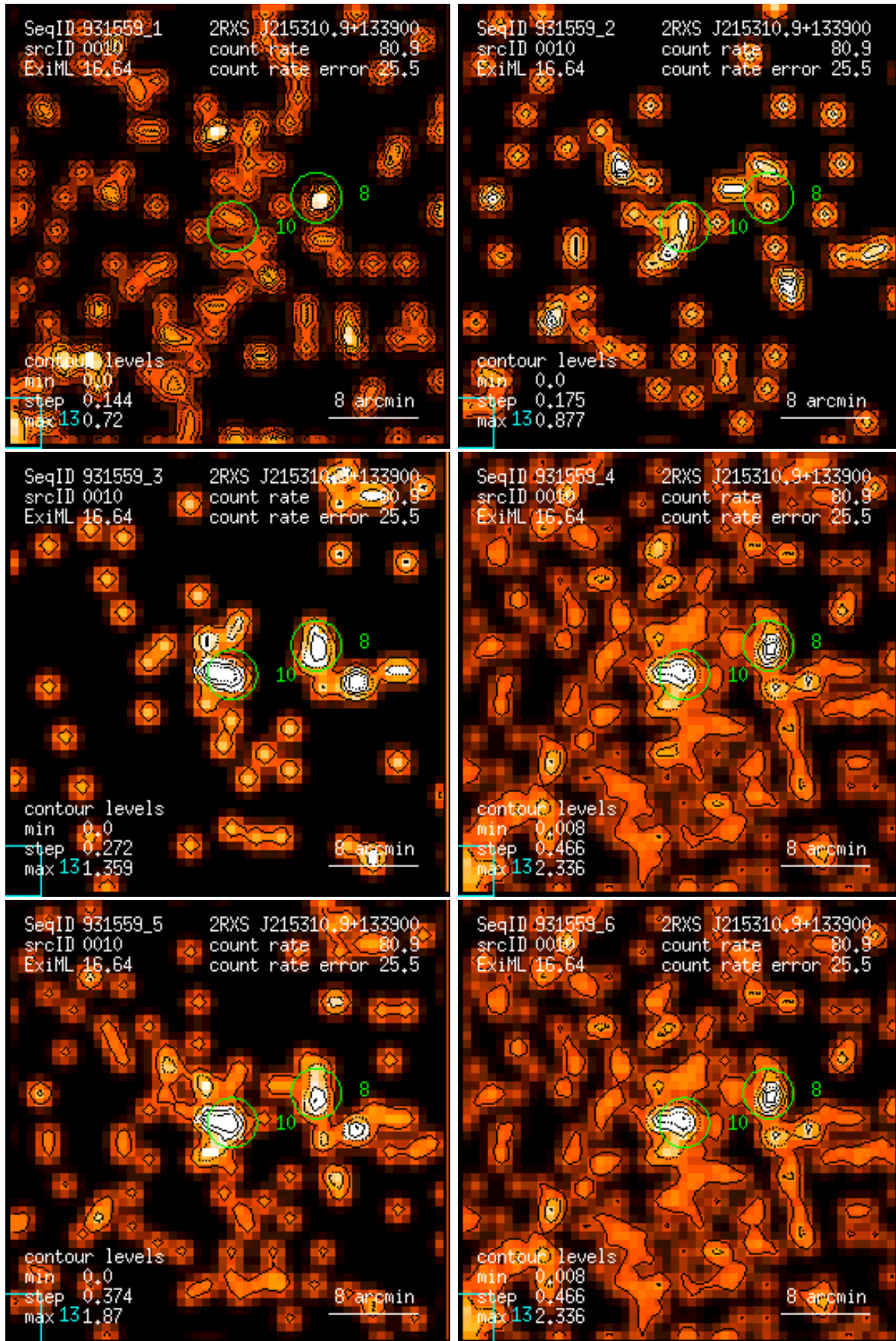
Figure 10: RASS 931559: detection 0010: band rate images, Gaussian filter: (1) PSPC channels 11 – 41, (2) 52 – 90, (3) 91 – 201, (4) 11 – 235, (5) 52 – 201, (6) 11 – 201. Broad band rates in counts/ks. Band rate contour levels in counts/ks/arcmin 2 .
