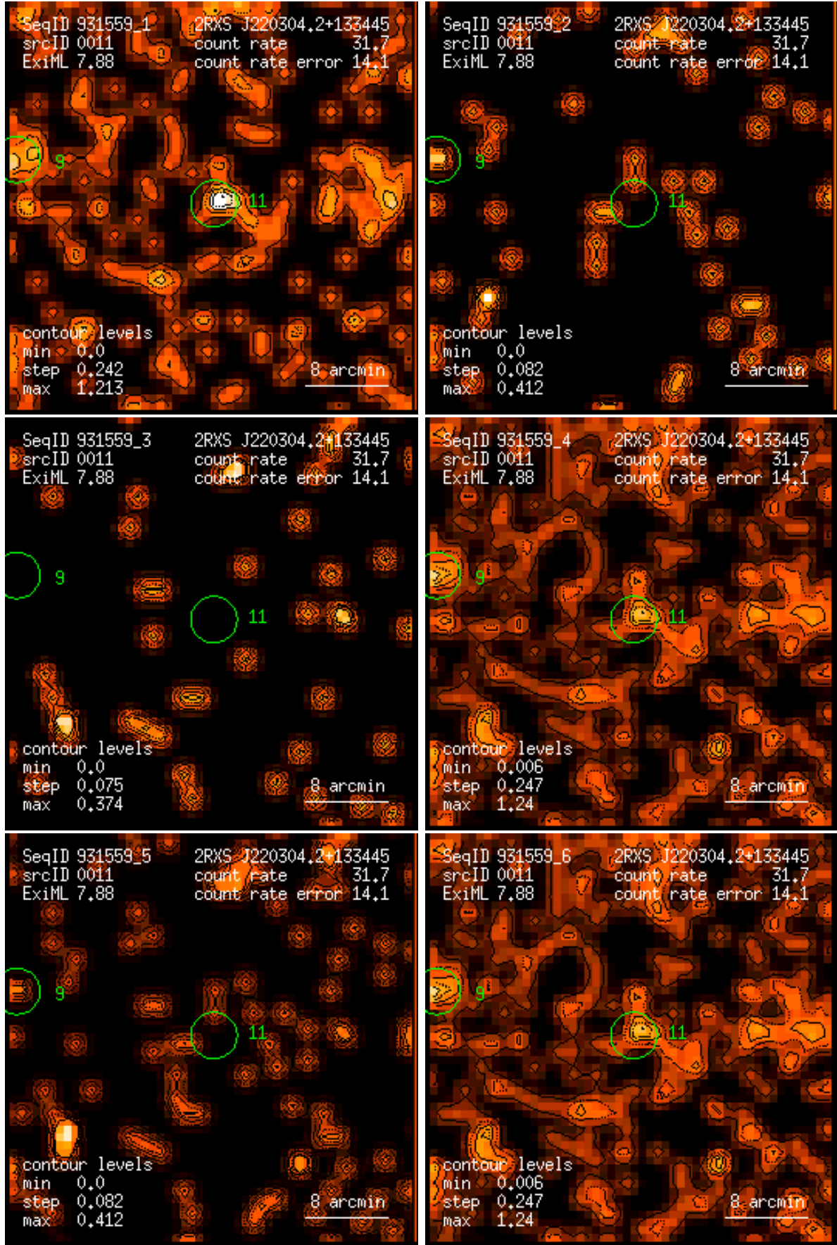
Figure 11: RASS 931559: detection 0011: band rate images, Gaussian filter: (1) PSPC channels 11 – 41, (2) 52 – 90, (3) 91 – 201, (4) 11 – 235, (5) 52 – 201, (6) 11 – 201. Broad band rates in counts/ks. Band rate contour levels in counts/ks/arcmin 2 .
