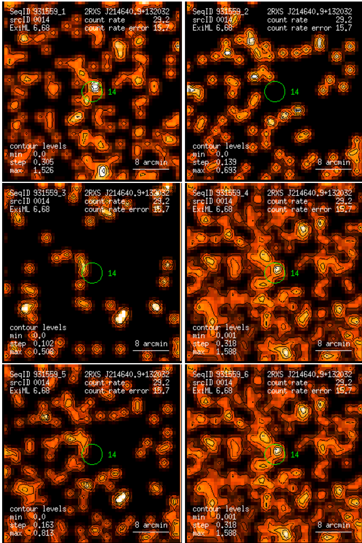
Figure 14: RASS 931559: detection 0014: band rate images, Gaussian filter: (1) PSPC channels 11 – 41, (2) 52 – 90, (3) 91 – 201, (4) 11 – 235, (5) 52 – 201, (6) 11 – 201. Broad band rates in counts/ks. Band rate contour levels in counts/ks/arcmin 2 .
