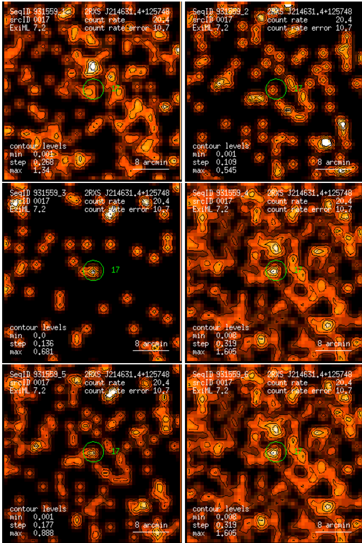
Figure 17: RASS 931559: detection 0017: band rate images, Gaussian filter: (1) PSPC channels 11 – 41, (2) 52 – 90, (3) 91 – 201, (4) 11 – 235, (5) 52 – 201, (6) 11 – 201. Broad band rates in counts/ks. Band rate contour levels in counts/ks/arcmin 2 .
