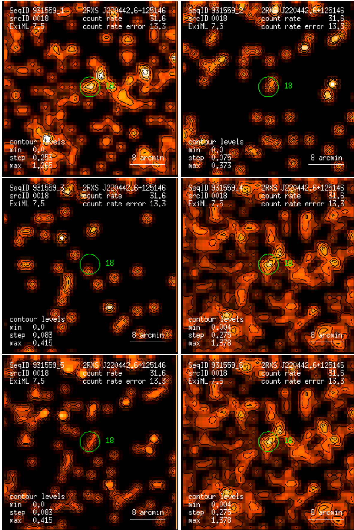
Figure 18: RASS 931559: detection 0018: band rate images, Gaussian filter: (1) PSPC channels 11 – 41, (2) 52 – 90, (3) 91 – 201, (4) 11 – 235, (5) 52 – 201, (6) 11 – 201. Broad band rates in counts/ks. Band rate contour levels in counts/ks/arcmin 2 .
