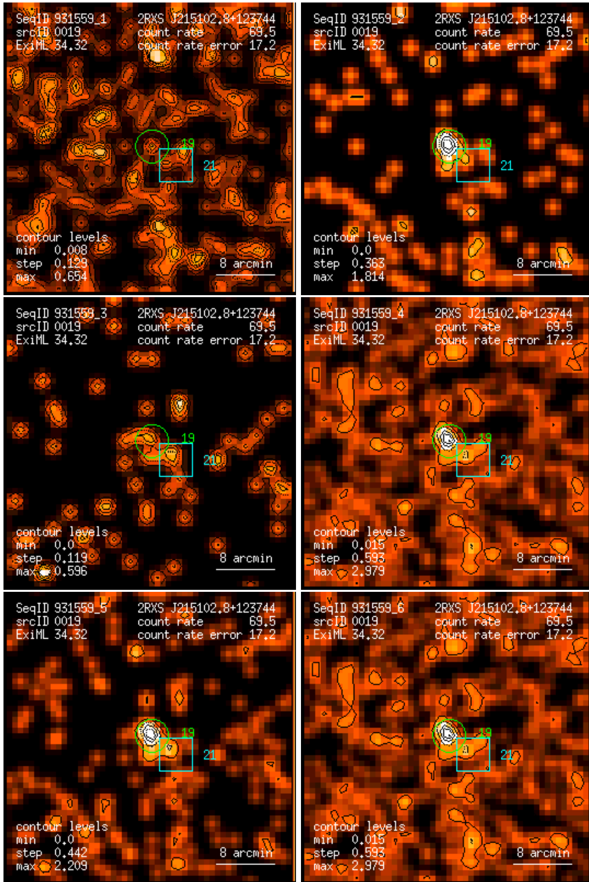
Figure 19: RASS 931559: detection 0019: band rate images, Gaussian filter: (1) PSPC channels 11 – 41, (2) 52 – 90, (3) 91 – 201, (4) 11 – 235, (5) 52 – 201, (6) 11 – 201. Broad band rates in counts/ks. Band rate contour levels in counts/ks/arcmin 2 .
