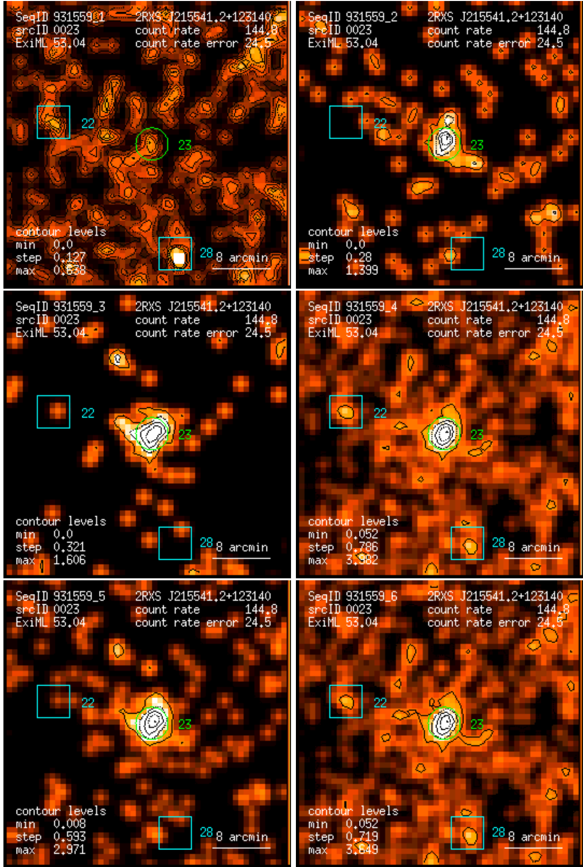
Figure 23: RASS 931559: detection 0023: band rate images, Gaussian filter: (1) PSPC channels 11 – 41, (2) 52 – 90, (3) 91 – 201, (4) 11 – 235, (5) 52 – 201, (6) 11 – 201. Broad band rates in counts/ks. Band rate contour levels in counts/ks/arcmin 2 .
