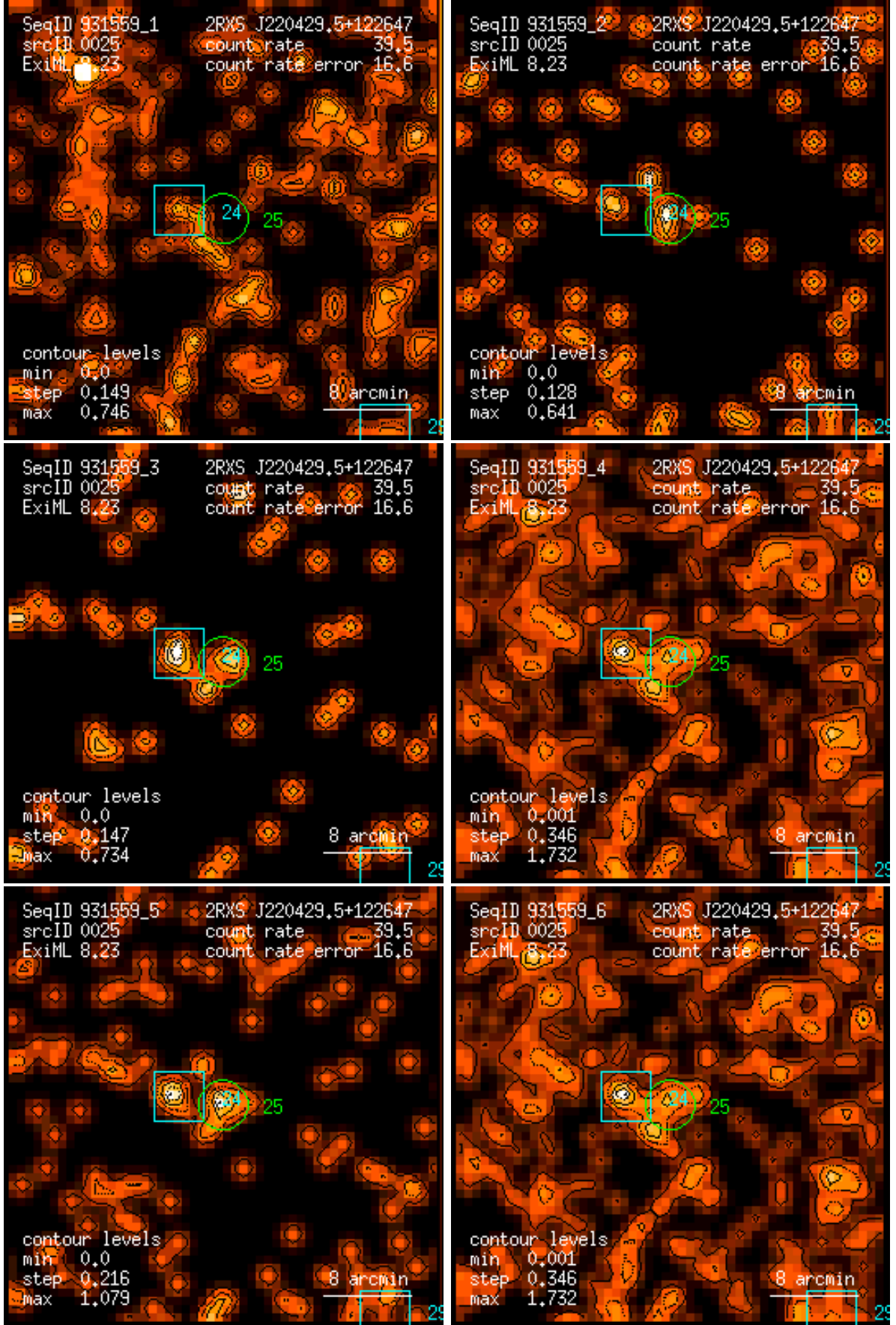
Figure 25: RASS 931559: detection 0025: band rate images, Gaussian filter: (1) PSPC channels 11 – 41, (2) 52 – 90, (3) 91 – 201, (4) 11 – 235, (5) 52 – 201, (6) 11 – 201. Broad band rates in counts/ks. Band rate contour levels in counts/ks/arcmin 2 .
