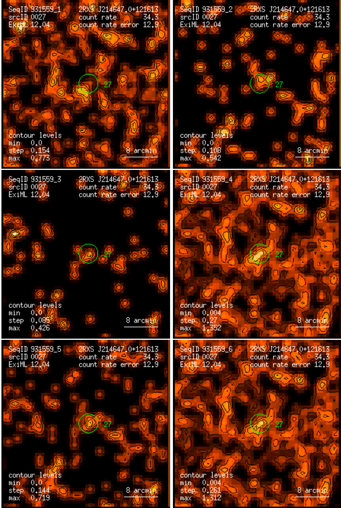
Figure 27: RASS 931559: detection 0027: band rate images, Gaussian filter: (1) PSPC channels 11 – 41, (2) 52 – 90, (3) 91 – 201, (4) 11 – 235, (5) 52 – 201, (6) 11 – 201. Broad band rates in counts/ks. Band rate contour levels in counts/ks/arcmin 2 .
