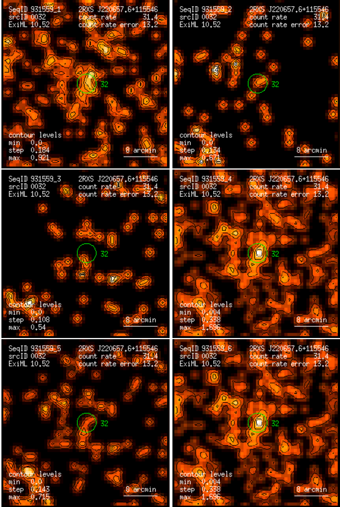
Figure 32: RASS 931559: detection 0032: band rate images, Gaussian filter: (1) PSPC channels 11 – 41, (2) 52 – 90, (3) 91 – 201, (4) 11 – 235, (5) 52 – 201, (6) 11 – 201. Broad band rates in counts/ks. Band rate contour levels in counts/ks/arcmin 2 .
