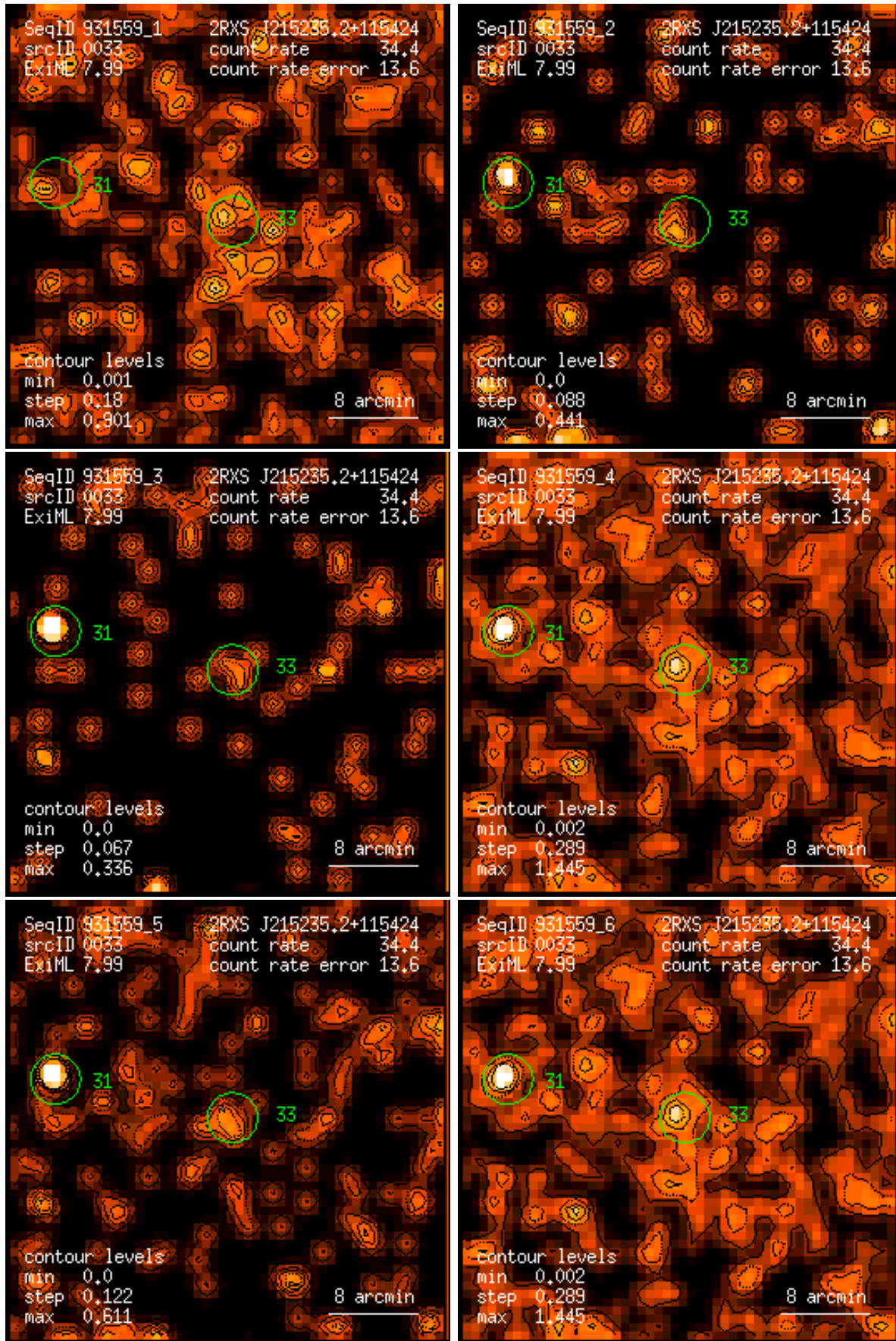
Figure 33: RASS 931559: detection 0033: band rate images, Gaussian filter: (1) PSPC channels 11 – 41, (2) 52 – 90, (3) 91 – 201, (4) 11 – 235, (5) 52 – 201, (6) 11 – 201. Broad band rates in counts/ks. Band rate contour levels in counts/ks/arcmin 2 .
