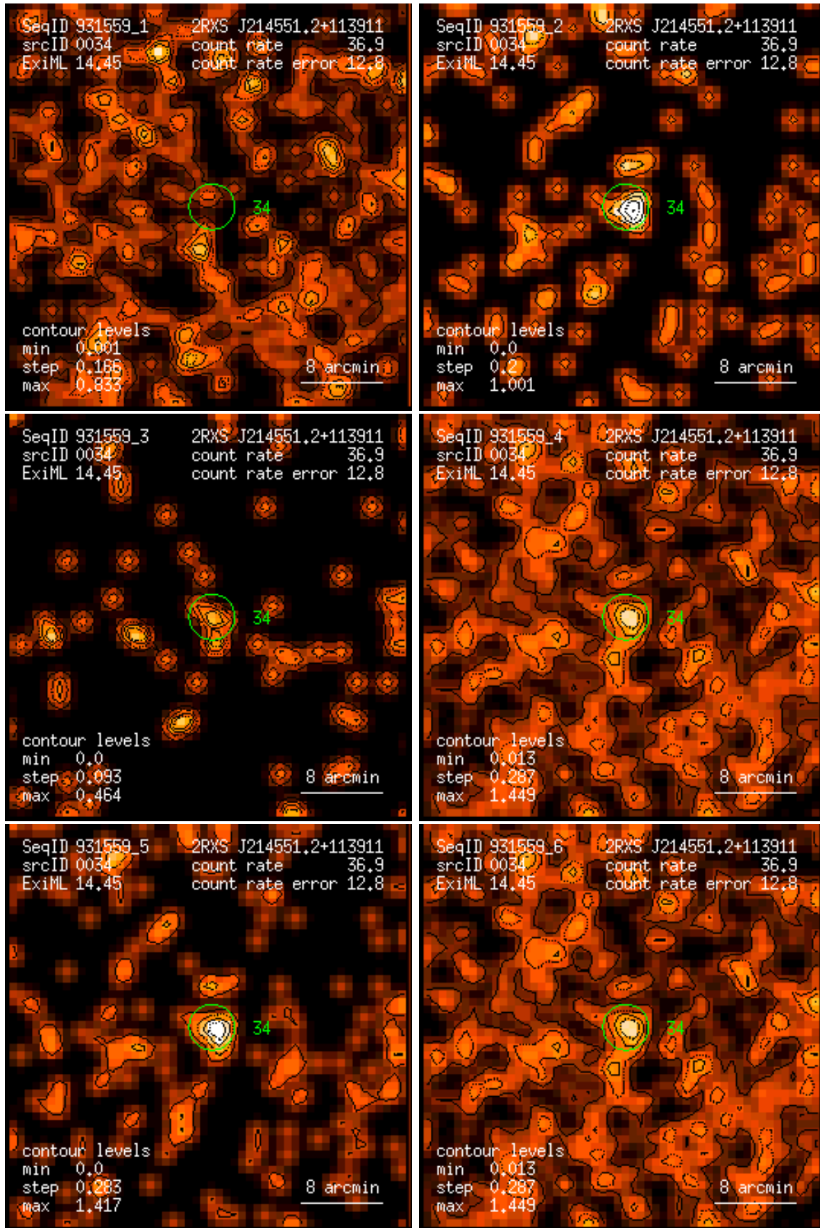
Figure 34: RASS 931559: detection 0034: band rate images, Gaussian filter: (1) PSPC channels 11 – 41, (2) 52 – 90, (3) 91 – 201, (4) 11 – 235, (5) 52 – 201, (6) 11 – 201. Broad band rates in counts/ks. Band rate contour levels in counts/ks/arcmin 2 .
