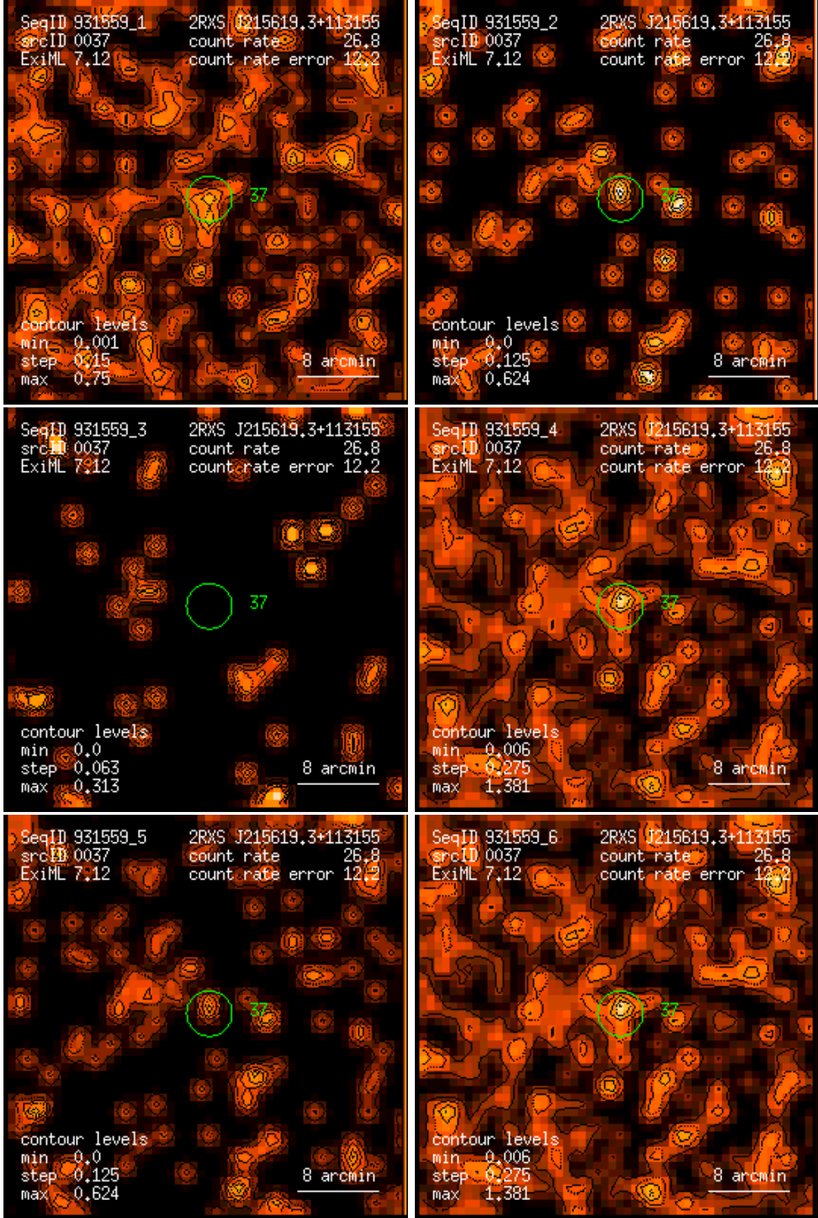
Figure 37: RASS 931559: detection 0037: band rate images, Gaussian filter: (1) PSPC channels 11 – 41, (2) 52 – 90, (3) 91 – 201, (4) 11 – 235, (5) 52 – 201, (6) 11 – 201. Broad band rates in counts/ks. Band rate contour levels in counts/ks/arcmin 2 .
