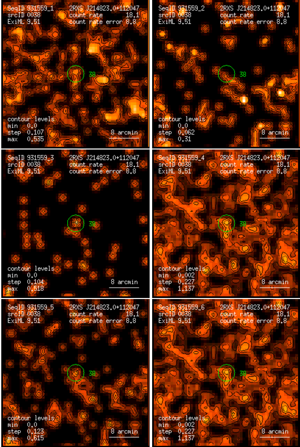
Figure 38: RASS 931559: detection 0038: band rate images, Gaussian filter: (1) PSPC channels 11 – 41, (2) 52 – 90, (3) 91 – 201, (4) 11 – 235, (5) 52 – 201, (6) 11 – 201. Broad band rates in counts/ks. Band rate contour levels in counts/ks/arcmin 2 .
