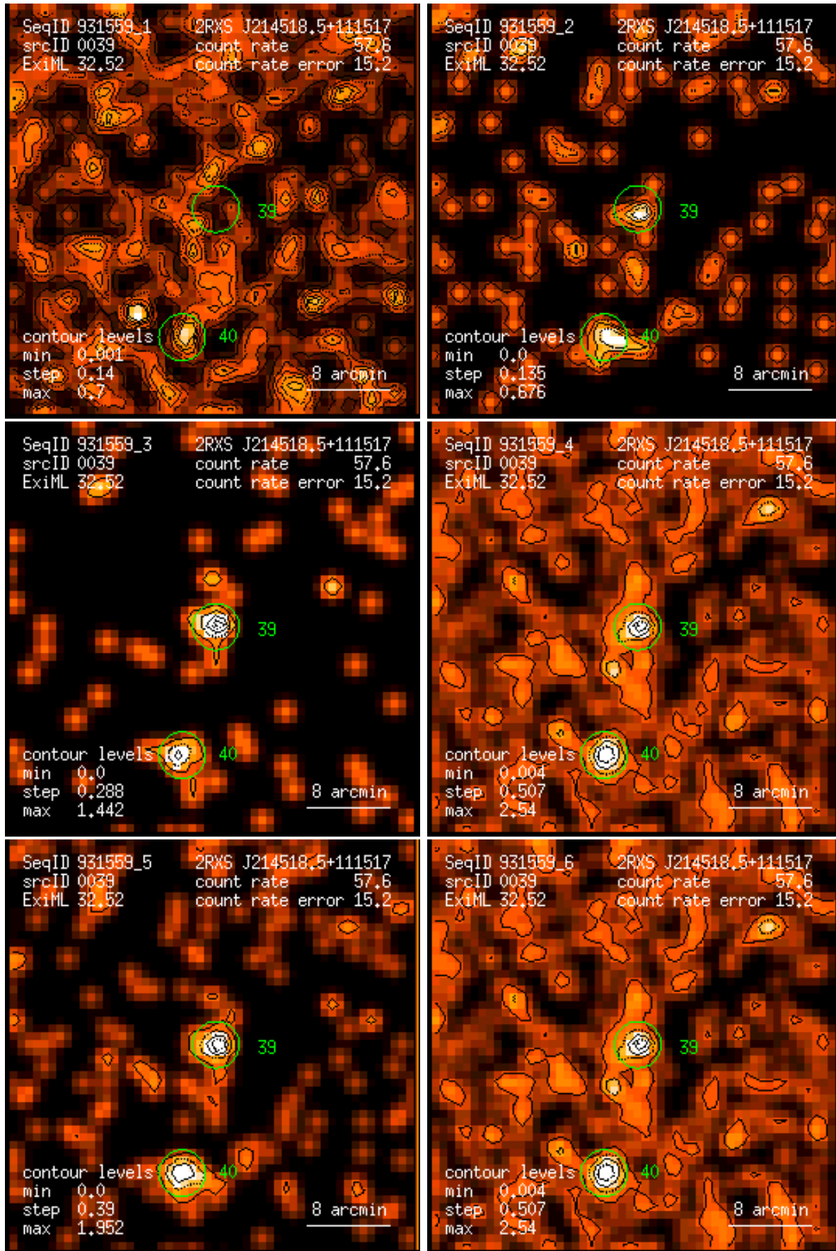
Figure 39: RASS 931559: detection 0039: band rate images, Gaussian filter: (1) PSPP channels 11 – 41, (2) 52 – 90, (3) 91 – 201, (4) 11 – 235, (5) 52 – 201, (6) 11 – 201. Broad band rates in counts/ks. Band rate contour levels in counts/ks/arcmin 2 .
