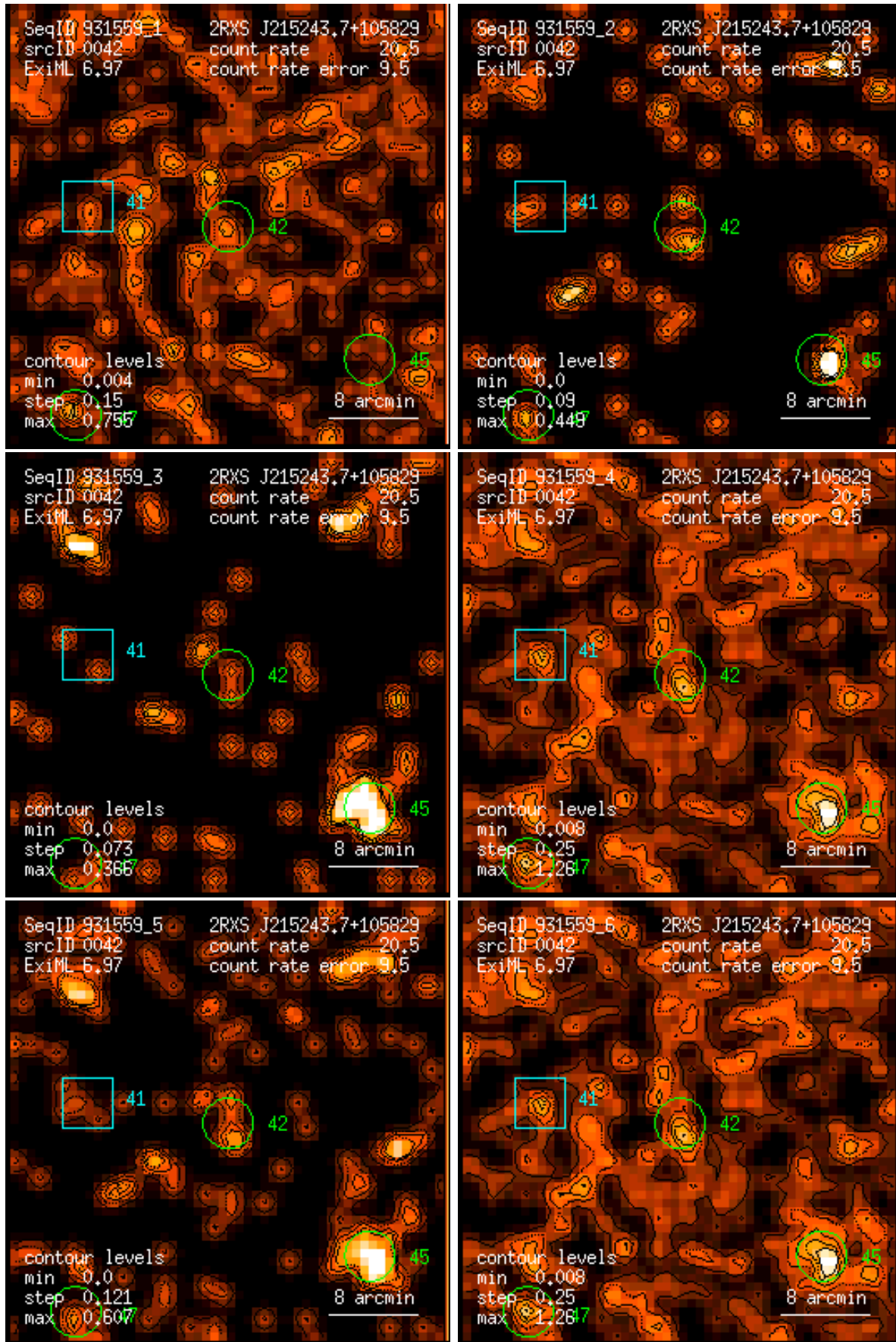
Figure 42: RASS 931559: detection 0042: band rate images, Gaussian filter: (1) PSPC channels 11 – 41, (2) 52 – 90, (3) 91 – 201, (4) 11 – 235, (5) 52 – 201, (6) 11 – 201. Broad band rates in counts/ks. Band rate contour levels in counts/ks/arcmin 2 .
