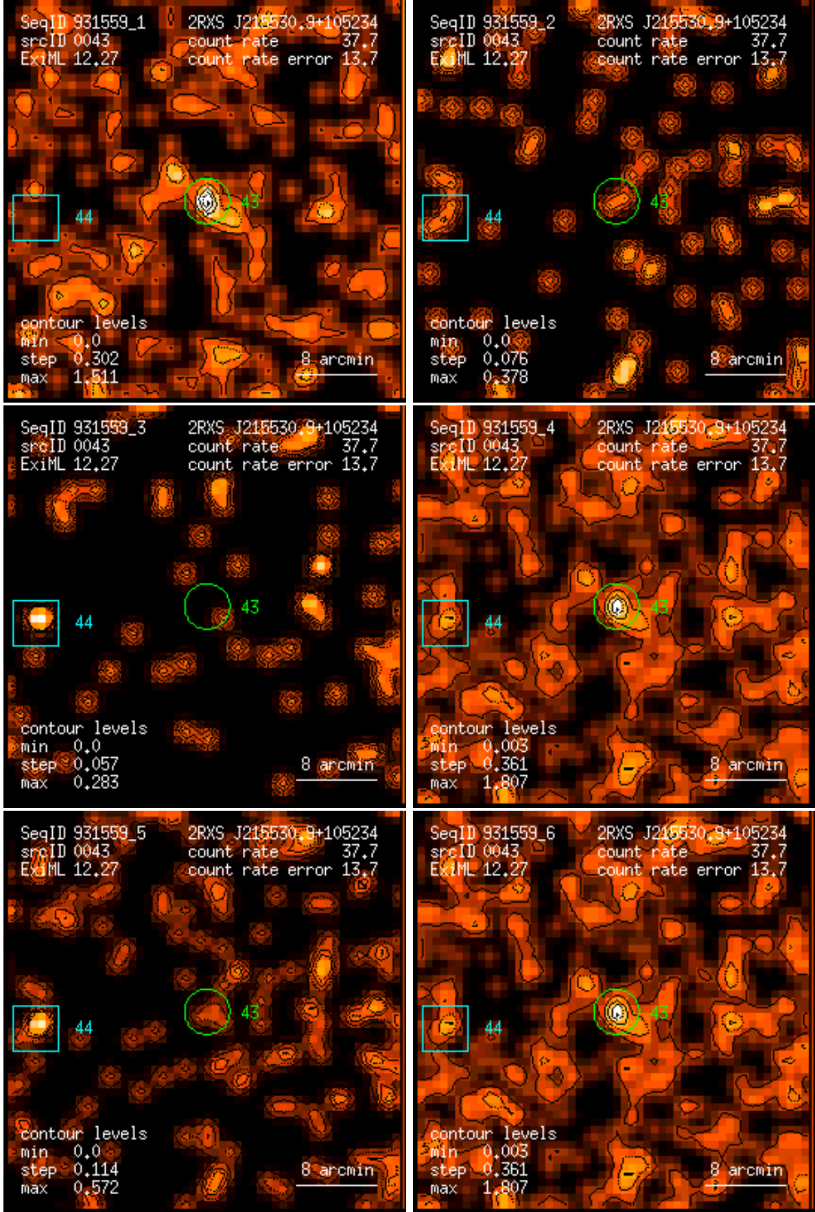
Figure 43: RASS 931559: detection 0043: band rate images, Gaussian filter: (1) PSPC channels 11 – 41, (2) 52 – 90, (3) 91 – 201, (4) 11 – 235, (5) 52 – 201, (6) 11 – 201. Broad band rates in counts/ks. Band rate contour levels in counts/ks/arcmin 2 .
