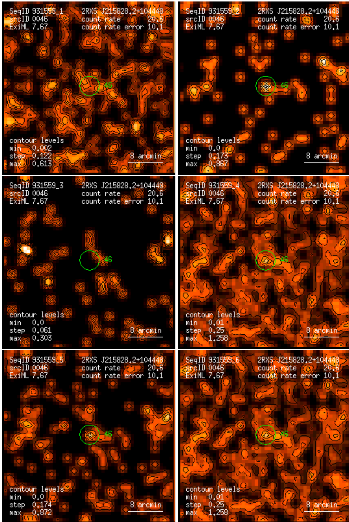
Figure 46: RASS 931559: detection 0046: band rate images, Gaussian filter: (1) PSPC channels 11 – 41, (2) 52 – 90, (3) 91 – 201, (4) 11 – 235, (5) 52 – 201, (6) 11 – 201. Broad band rates in counts/ks. Band rate contour levels in counts/ks/arcmin 2 .
