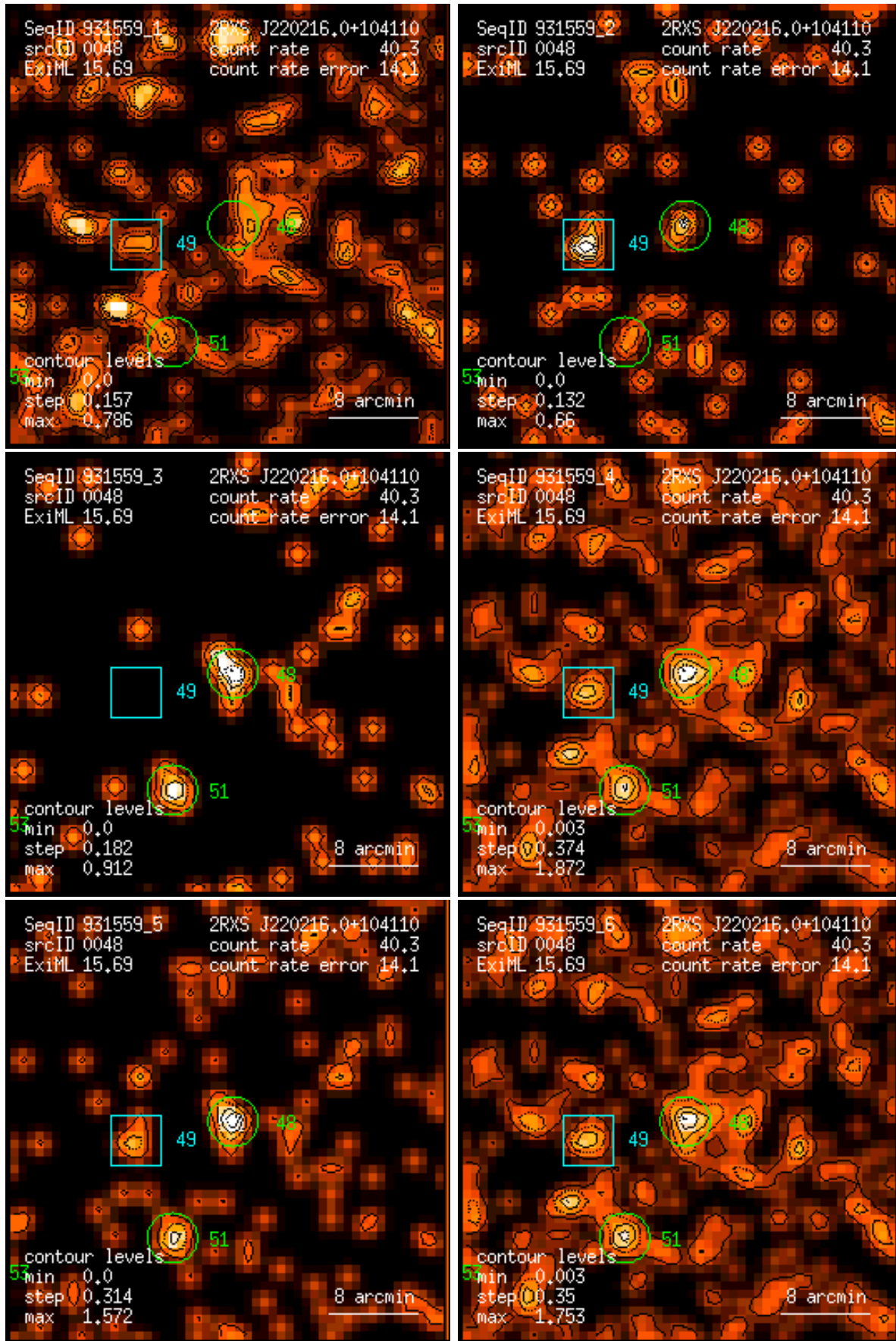
Figure 48: RASS 931559: detection 0048: band rate images, Gaussian filter: (1) PSPC channels 11 – 41, (2) 52 – 90, (3) 91 – 201, (4) 11 – 235, (5) 52 – 201, (6) 11 – 201. Broad band rates in counts/ks. Band rate contour levels in counts/ks/arcmin 2 .
