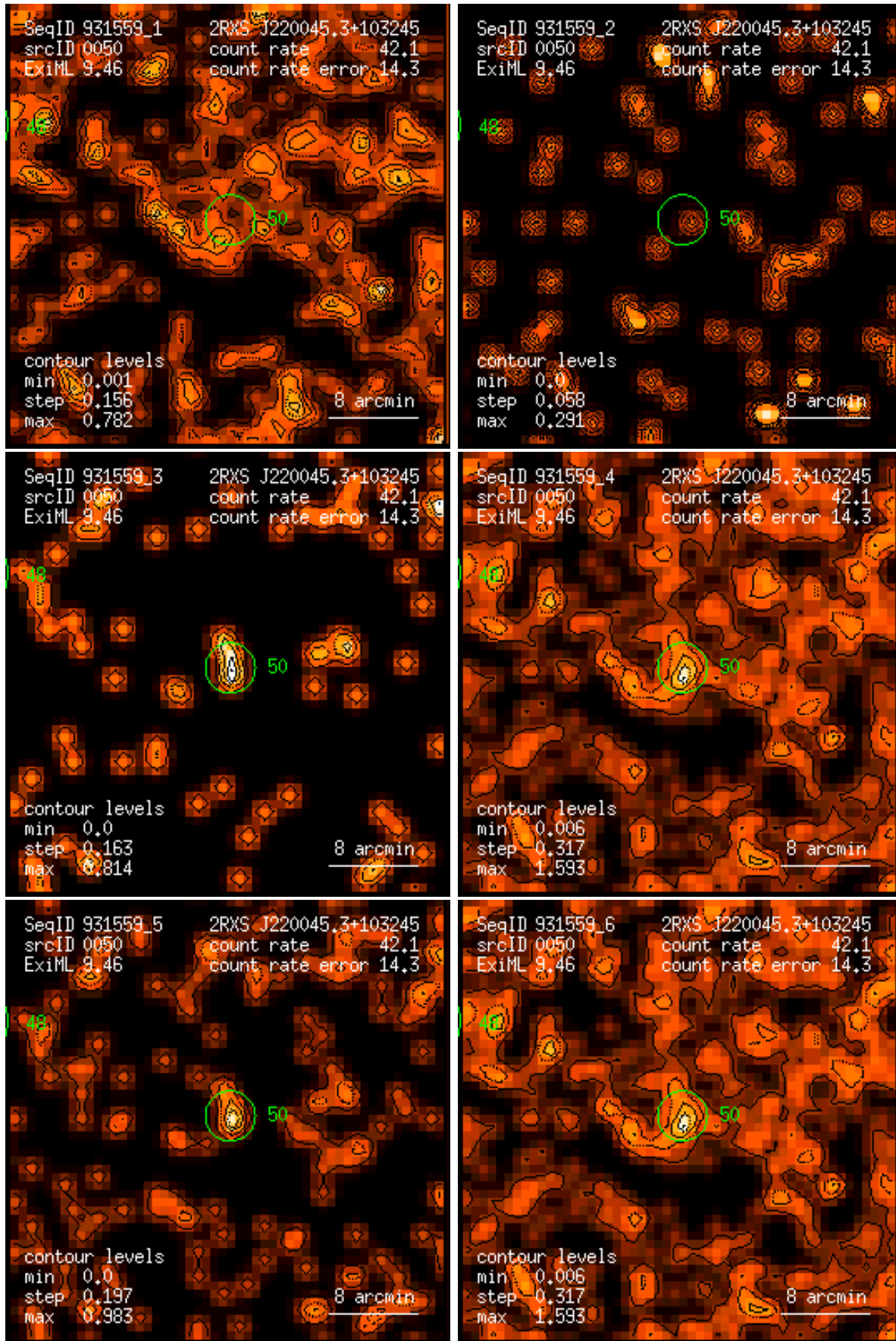
Figure 50: RASS 931559: detection 0050: band rate images, Gaussian filter: (1) PSPC channels 11 – 41, (2) 52 – 90, (3) 91 – 201, (4) 11 – 235, (5) 52 – 201, (6) 11 – 201. Broad band rates in counts/ks. Band rate contour levels in counts/ks/arcmin 2 .
