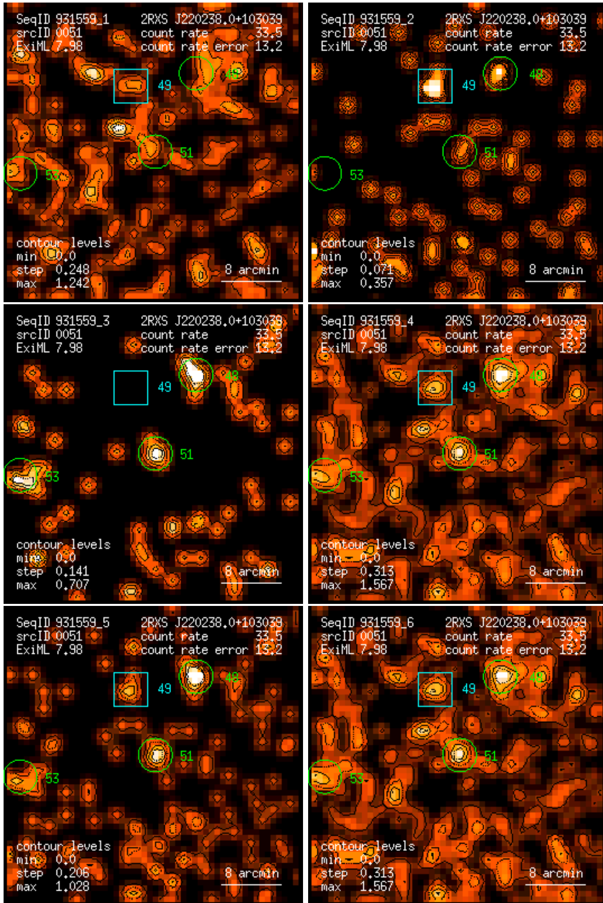
Figure 51: RASS 931559: detection 0051: band rate images, Gaussian filter: (1) PSPC channels 11 – 41, (2) 52 – 90, (3) 91 – 201, (4) 11 – 235, (5) 52 – 201, (6) 11 – 201. Broad band rates in counts/ks. Band rate contour levels in counts/ks/arcmin 2 .
