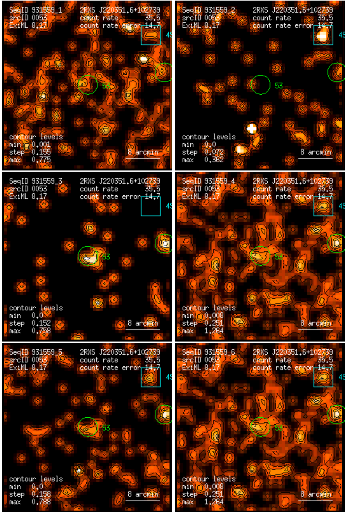
Figure 53: RASS 931559: detection 0053: band rate images, Gaussian filter: (1) PSPC channels 11 – 41, (2) 52 – 90, (3) 91 – 201, (4) 11 – 235, (5) 52 – 201, (6) 11 – 201. Broad band rates in counts/ks. Band rate contour levels in counts/ks/arcmin 2 .
