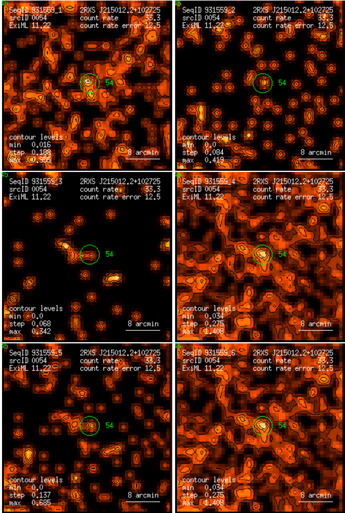
Figure 54: RASS 931559: detection 0054: band rate images, Gaussian filter: (1) PSPC channels 11 – 41, (2) 52 – 90, (3) 91 – 201, (4) 11 – 235, (5) 52 – 201, (6) 11 – 201. Broad band rates in counts/ks. Band rate contour levels in counts/ks/arcmin 2 .
