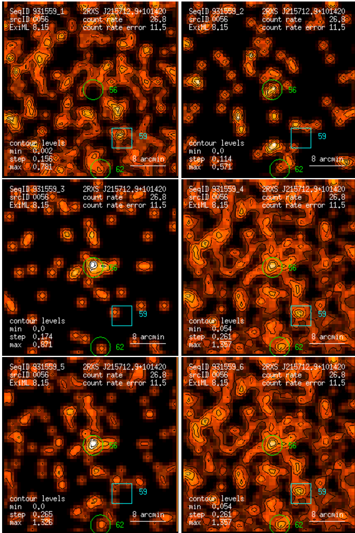
Figure 56: RASS 931559: detection 0056: band rate images, Gaussian filter: (1) PSPC channels 11 – 41, (2) 52 – 90, (3) 91 – 201, (4) 11 – 235, (5) 52 – 201, (6) 11 – 201. Broad band rates in counts/ks. Band rate contour levels in counts/ks/arcmin 2 .
