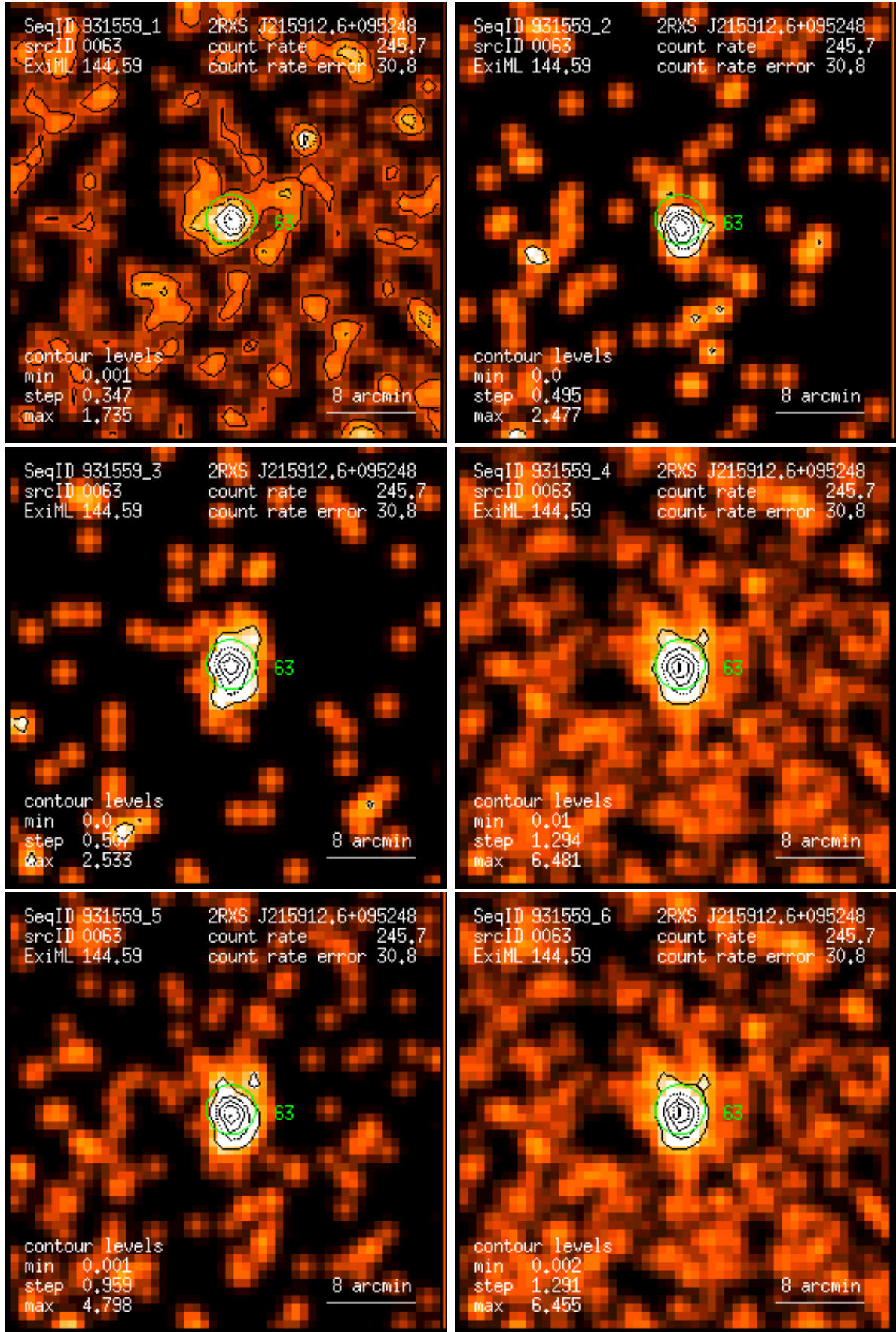
Figure 63: RASS 931559: detection 0063: band rate images, Gaussian filter: (1) PSPC channels 11 – 41, (2) 52 – 90, (3) 91 – 201, (4) 11 – 235, (5) 52 – 201, (6) 11 – 201. Broad band rates in counts/ks. Band rate contour levels in counts/ks/arcmin 2 .
