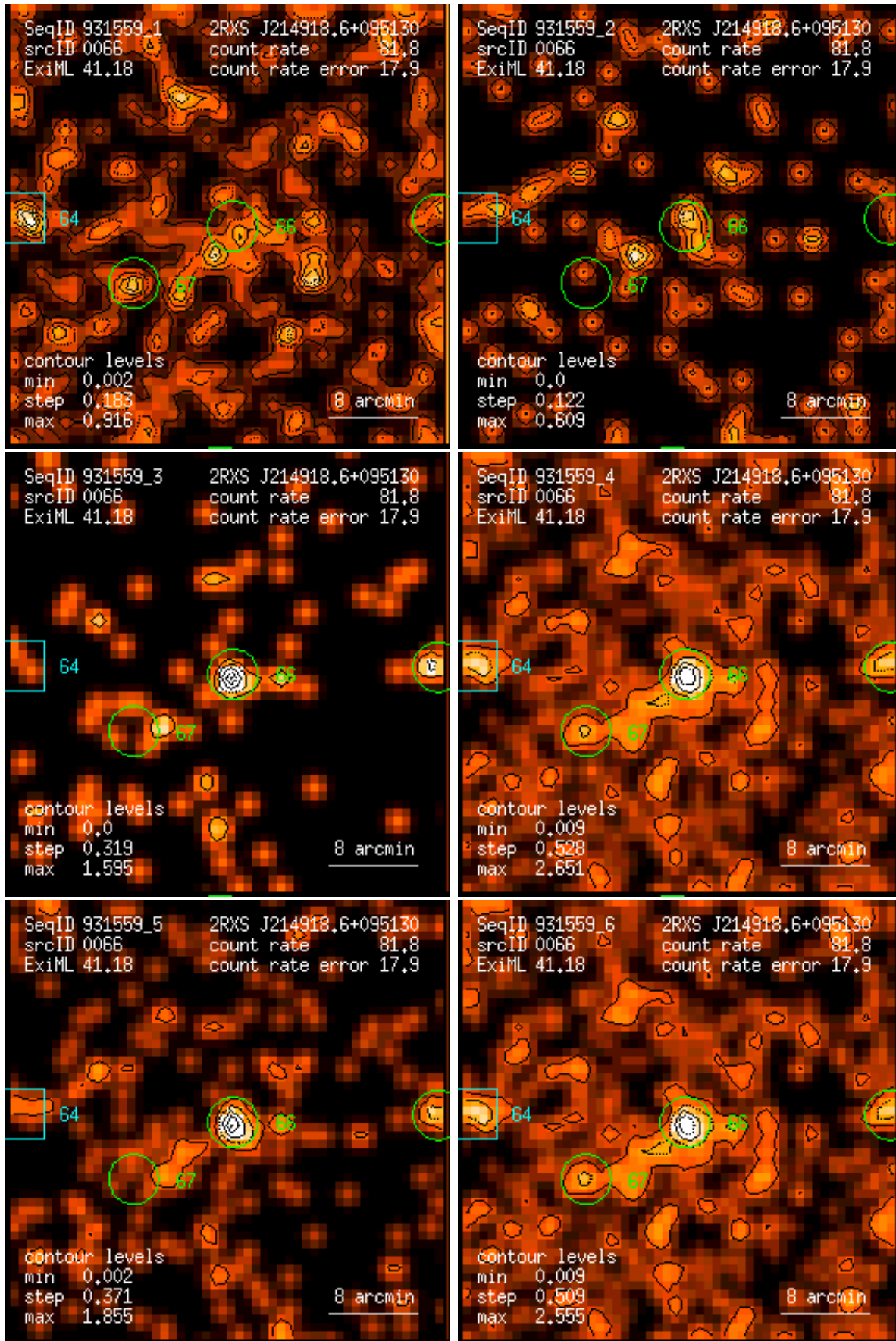
Figure 66: RASS 931559: detection 0066: band rate images, Gaussian filter: (1) PSPC channels 11 – 41, (2) 52 – 90, (3) 91 – 201, (4) 11 – 235, (5) 52 – 201, (6) 11 – 201. Broad band rates in counts/ks. Band rate contour levels in counts/ks/arcmin 2 .
