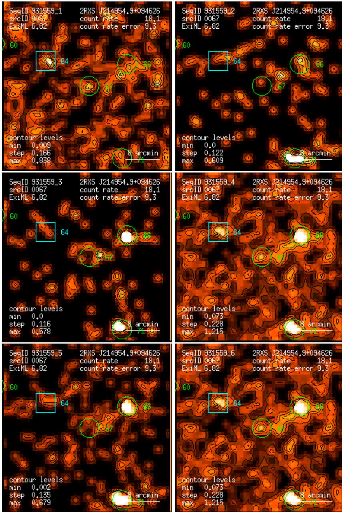
Figure 67: RASS 931559: detection 0067: band rate images, Gaussian filter: (1) PSPC channels 11 – 41, (2) 52 – 90, (3) 91 – 201, (4) 11 – 235, (5) 52 – 201, (6) 11 – 201. Broad band rates in counts/ks. Band rate contour levels in counts/ks/arcmin 2 .
