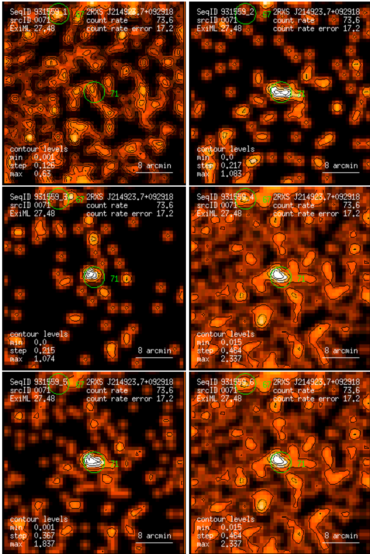
Figure 71: RASS 931559: detection 0071: band rate images, Gaussian filter: (1) PSPC channels 11 – 41, (2) 52 – 90, (3) 91 – 201, (4) 11 – 235, (5) 52 – 201, (6) 11 – 201. Broad band rates in counts/ks. Band rate contour levels in counts/ks/arcmin 2 .
