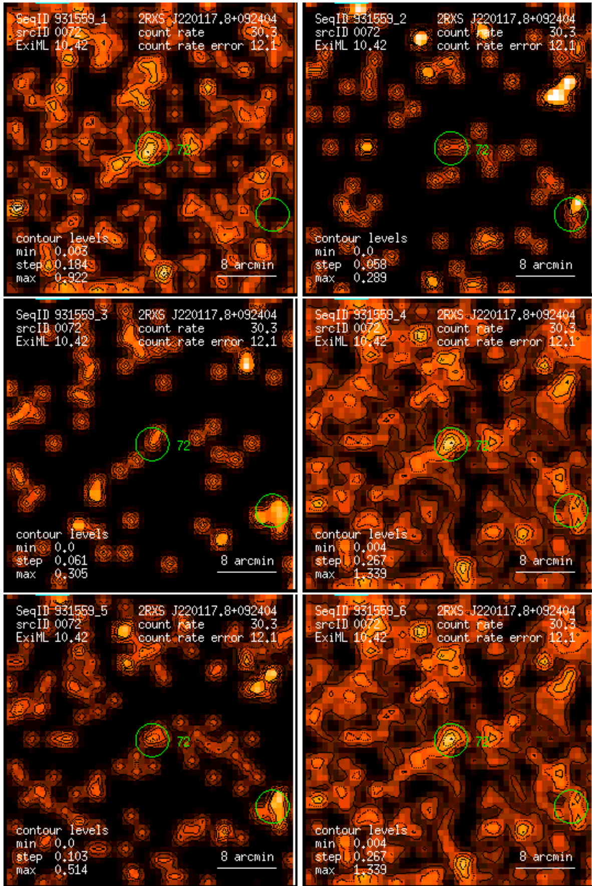
Figure 72: RASS 931559: detection 0072: band rate images, Gaussian filter: (1) PSPC channels 11 – 41, (2) 52 – 90, (3) 91 – 201, (4) 11 – 235, (5) 52 – 201, (6) 11 – 201. Broad band rates in counts/ks. Band rate contour levels in counts/ks/arcmin 2 .
