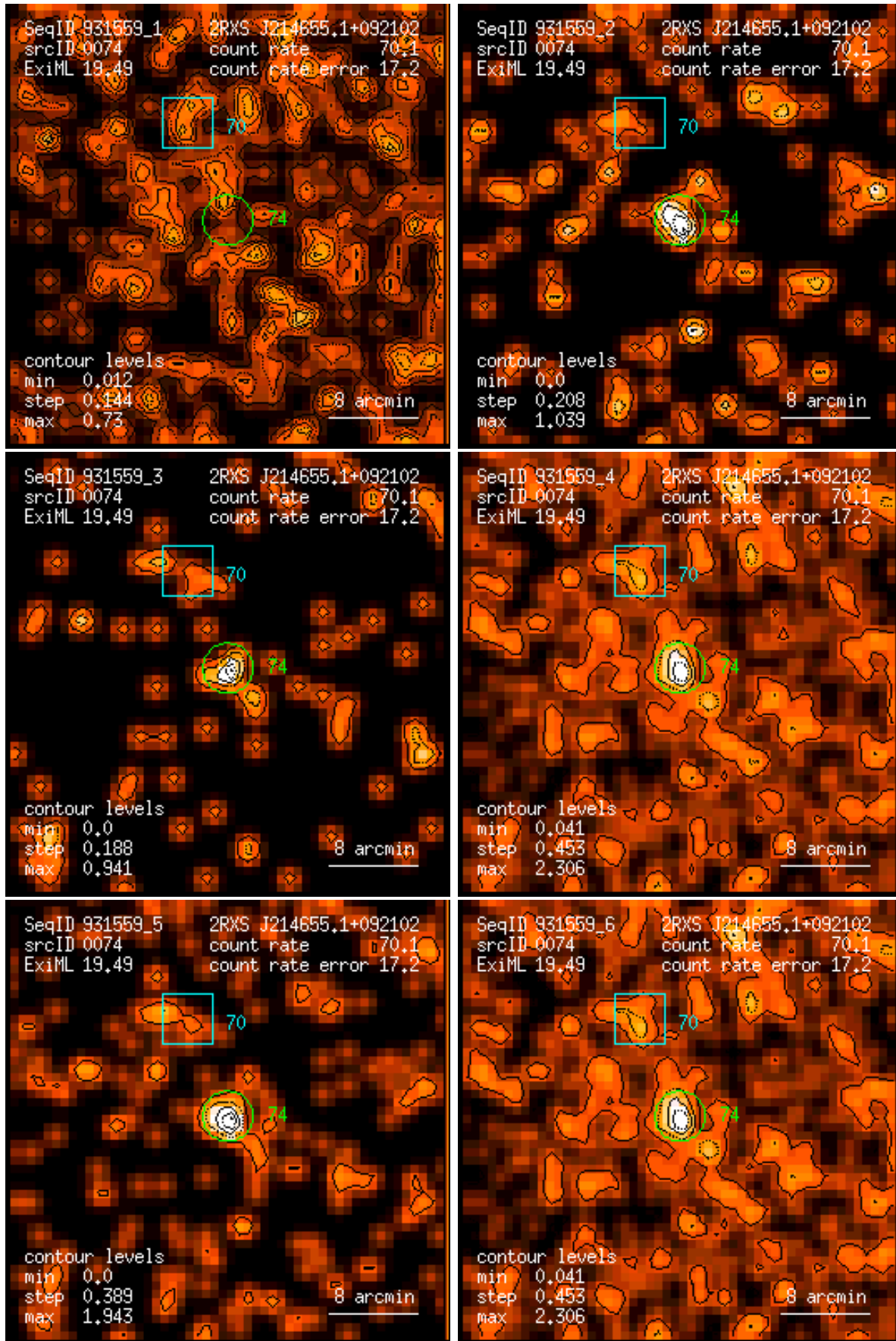
Figure 74: RASS 931559: detection 0074: band rate images, Gaussian filter: (1) PSPC channels 11 – 41, (2) 52 – 90, (3) 91 – 201, (4) 11 – 235, (5) 52 – 201, (6) 11 – 201. Broad band rates in counts/ks. Band rate contour levels in counts/ks/arcmin 2 .
