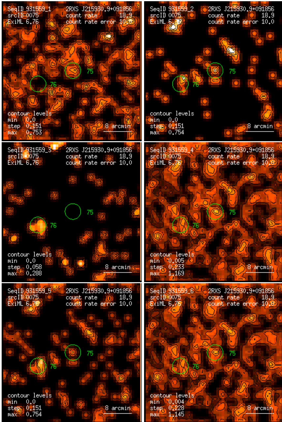
Figure 75: RASS 931559: detection 0075: band rate images, Gaussian filter: (1) PSPC channels 11 – 41, (2) 52 – 90, (3) 91 – 201, (4) 11 – 235, (5) 52 – 201, (6) 11 – 201. Broad band rates in counts/ks. Band rate contour levels in counts/ks/arcmin 2 .
