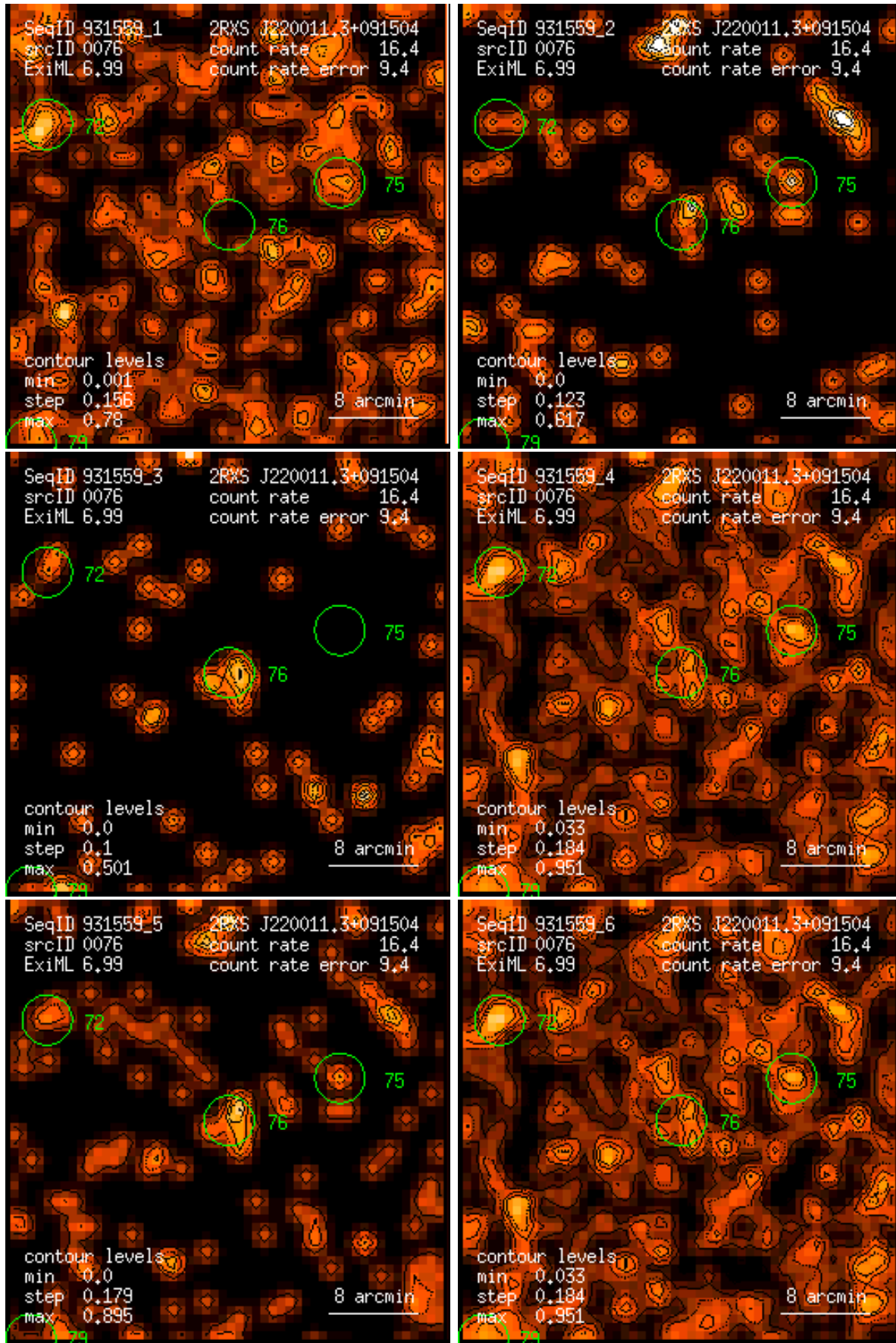
Figure 76: RASS 931559: detection 0076: band rate images, Gaussian filter: (1) PSPC channels 11 – 41, (2) 52 – 90, (3) 91 – 201, (4) 11 – 235, (5) 52 – 201, (6) 11 – 201. Broad band rates in counts/ks. Band rate contour levels in counts/ks/arcmin 2 .
