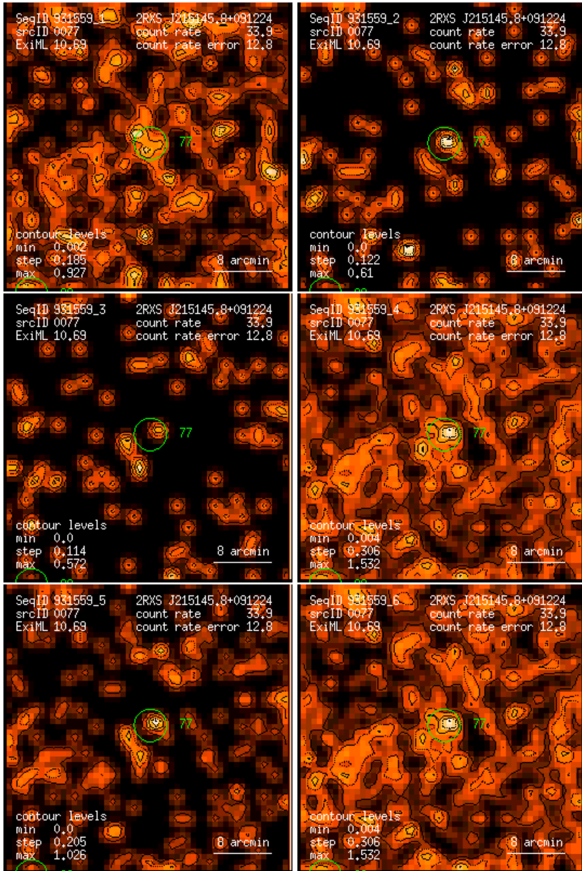
Figure 77: RASS 931559: detection 0077: band rate images, Gaussian filter: (1) PSPC channels 11 – 41, (2) 52 – 90, (3) 91 – 201, (4) 11 – 235, (5) 52 – 201, (6) 11 – 201. Broad band rates in counts/ks. Band rate contour levels in counts/ks/arcmin 2 .
